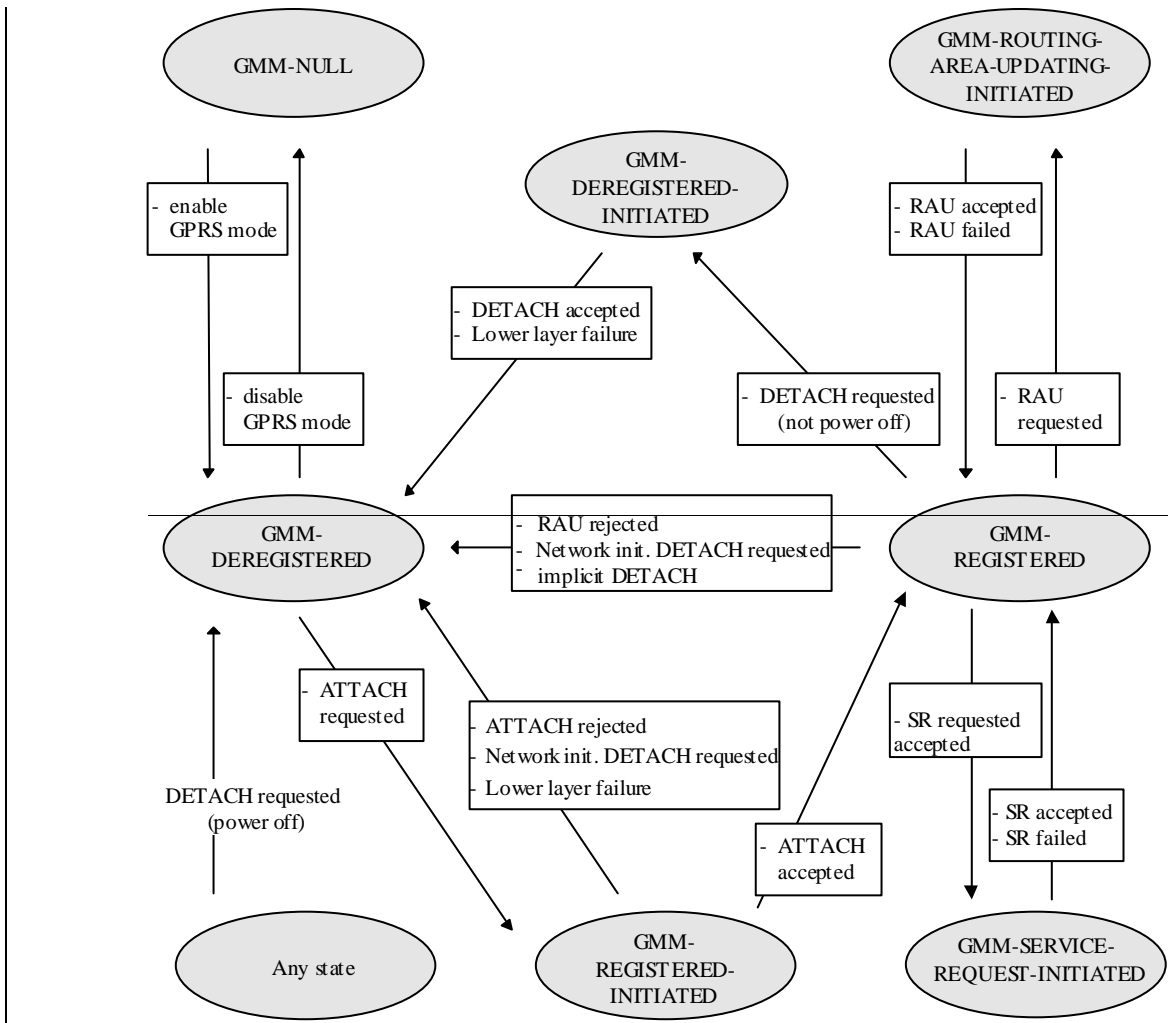
Figure 4.1b/3GPP TS 24.008:GMM main states in the MS
