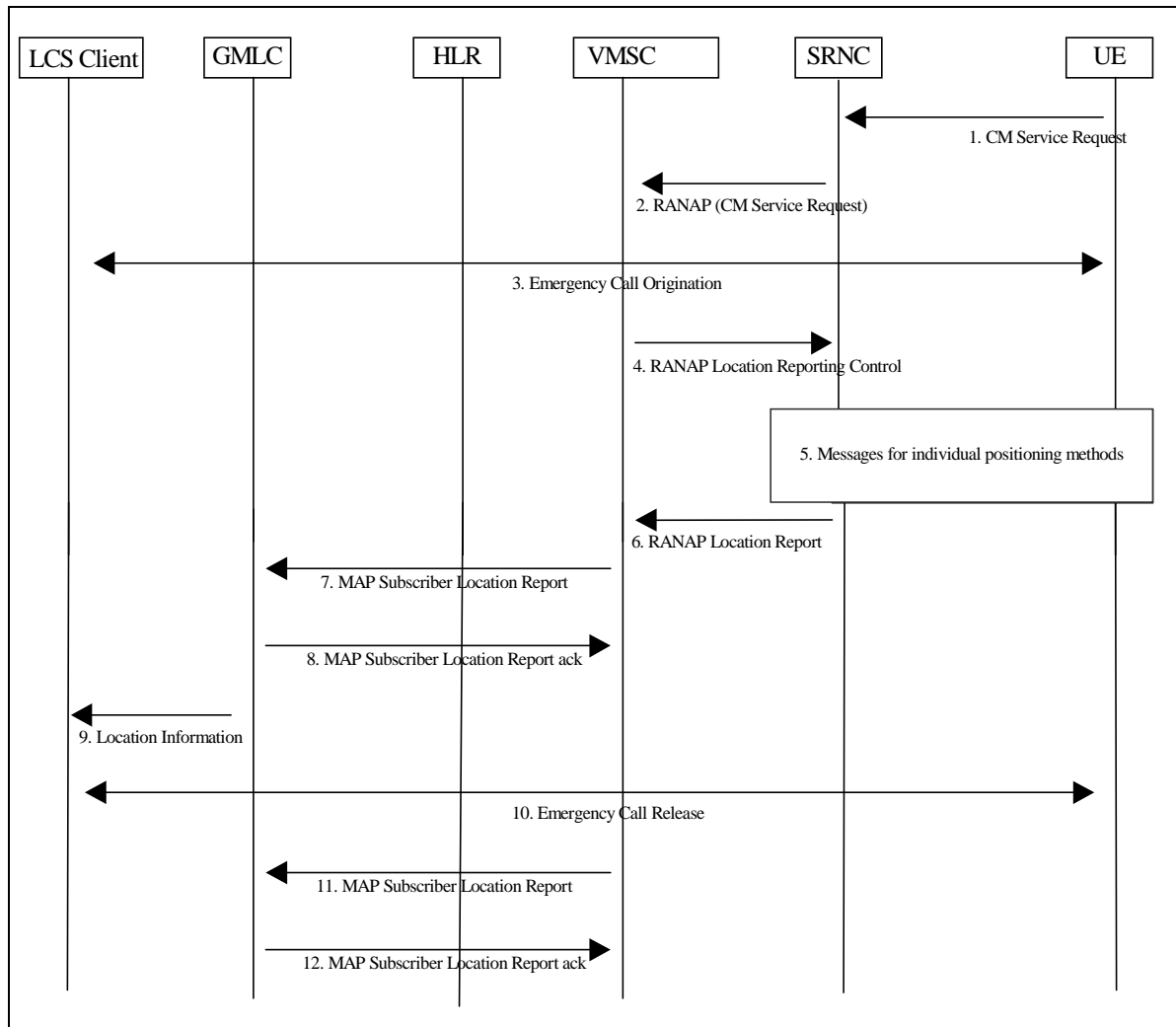
Figure 8.8 Positioning for a NI-LR Emergency Service Call
