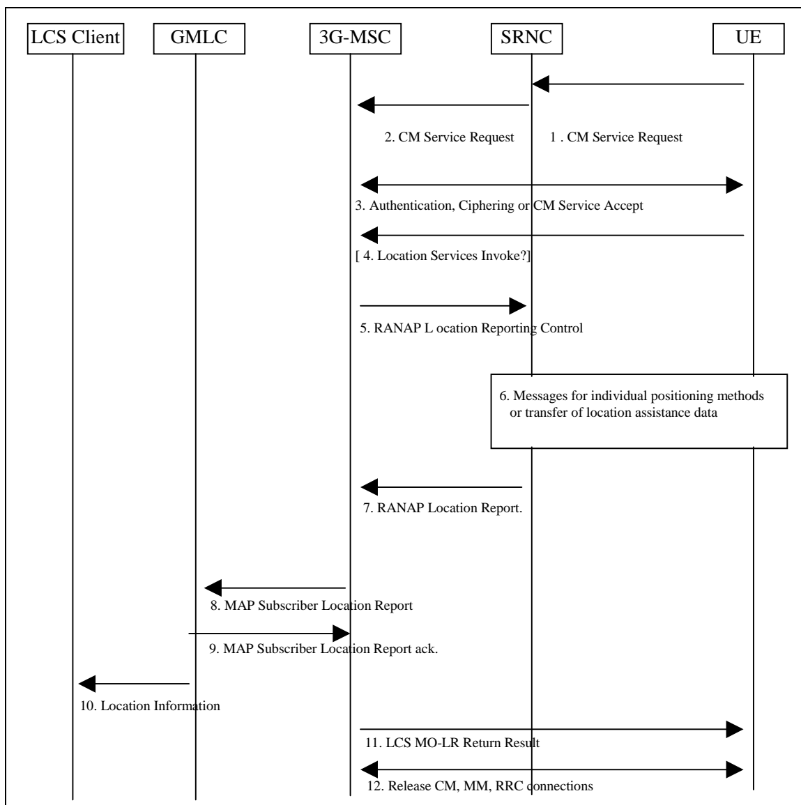
Figure 8.10 General Network Positioning for MO-LR
