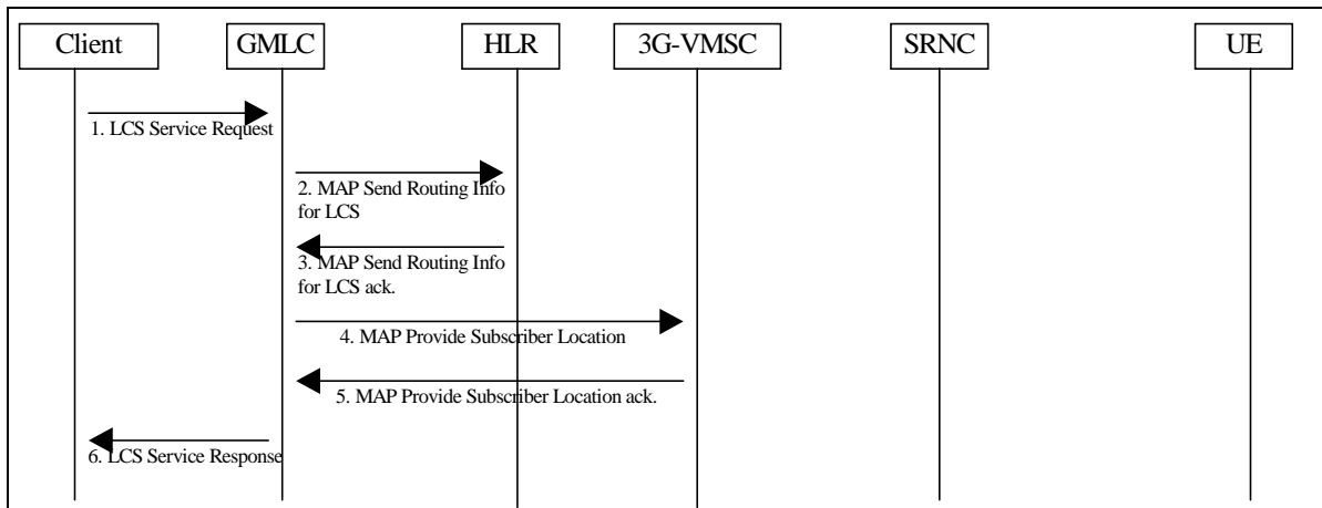
Figure 8.7 MT-LR for a previously obtained location estimate
