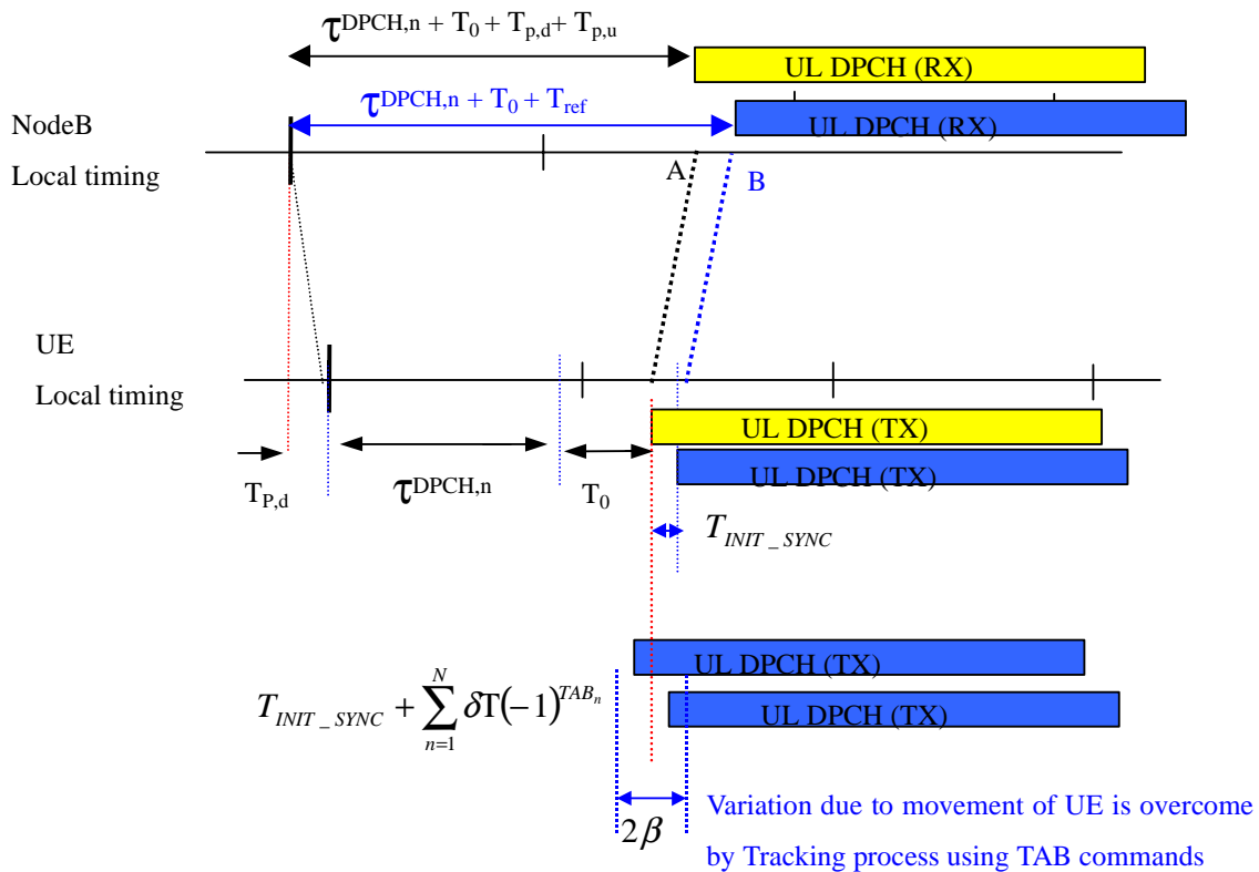
Figure 4.2 Initial synchronisation and Tracking process for DPDCH/DPCCH (Yellow: before adjustment, Blue: After adjustment).
