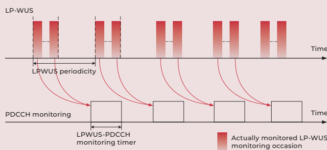
Figure 3 Option 2: LP-WUS operation in RRC connected modeoption 2
