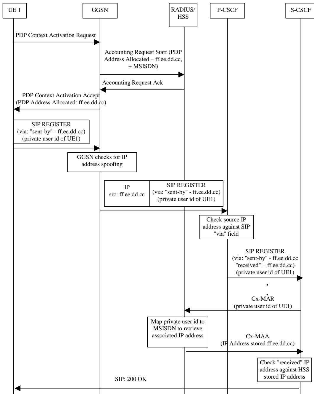
Figure 1 below describes the message flow for successful registration to the IMS that is specified by the interim security solution.
