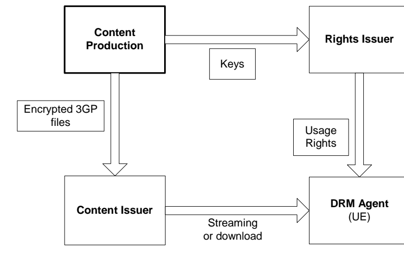
Figure 4: OMA DRM system architecture
