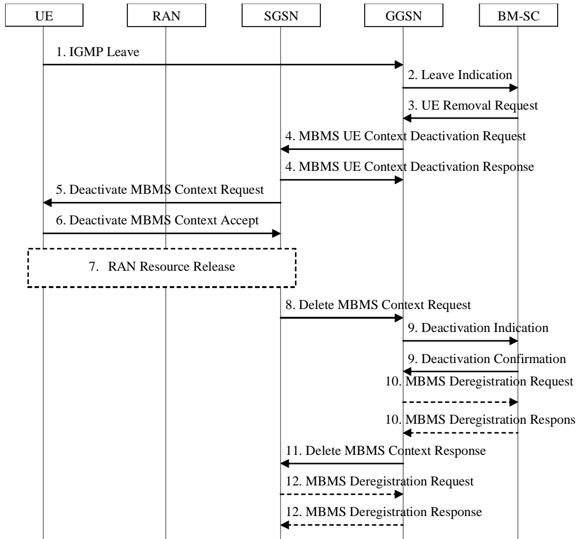
Figure 13: MBMS Multicast Service Deactivation
