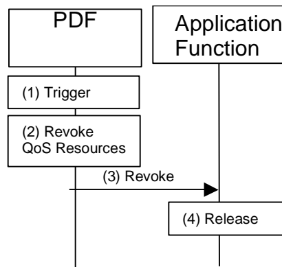
Figure 13: Revoke Session Authorization, PDF initiated
