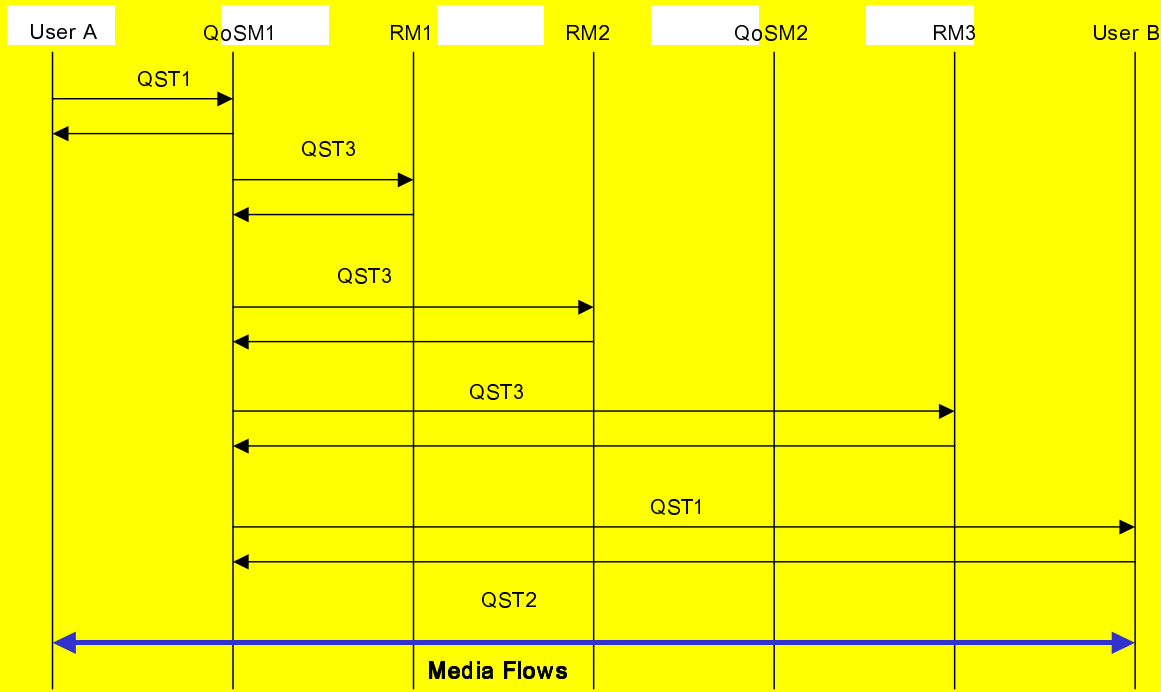
Figure 9 – QoS Signalling Option 1a
