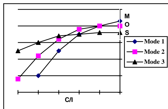
Fig. 5.2 - Family of curves showing performance for different codec modes
