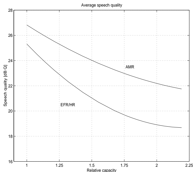
Fig. 6.1 - Average speech quality vs. relative capacity for AMR and EFR/HR
