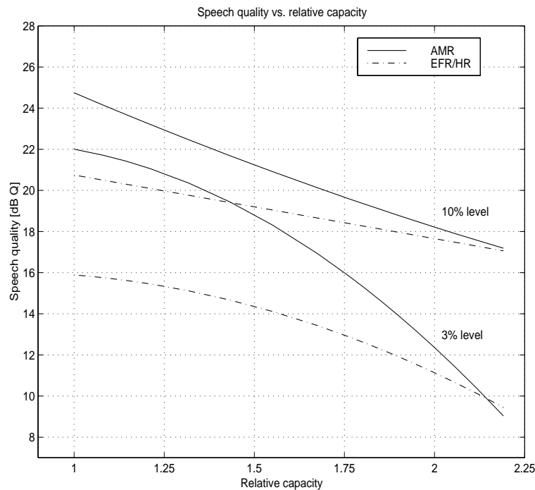
Fig. 6.2 - Speech quality for AMR and EFR/HR at the 3% and 10% levels
