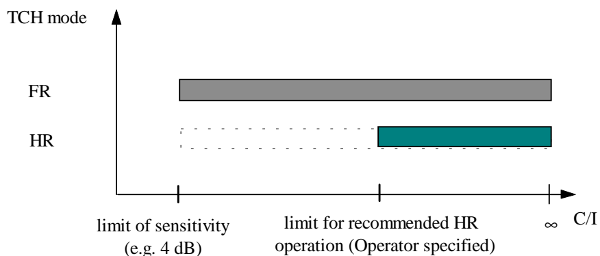
Fig. 5.1 - Preferred operating ranges for HR and FR channel modes.
