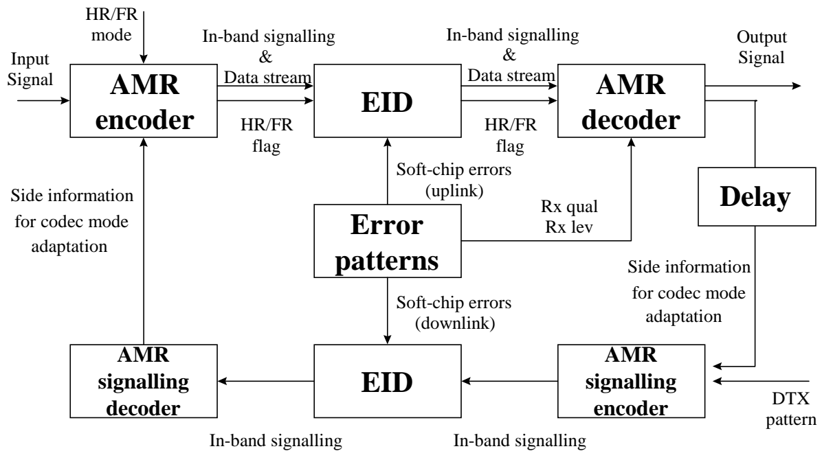
Fig. 9.1 - Block diagram of the AMR speech traffic channel simulation model.
