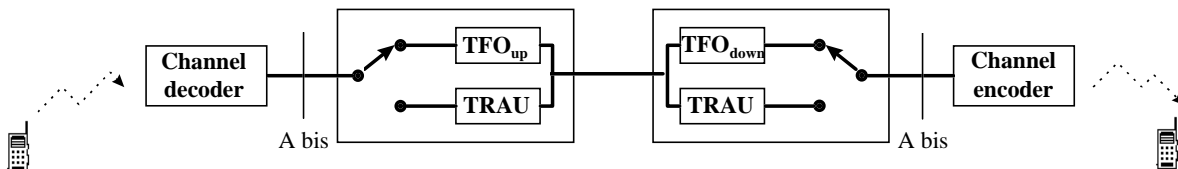
Fig. 6.4 - Mobile to mobile communication link.
