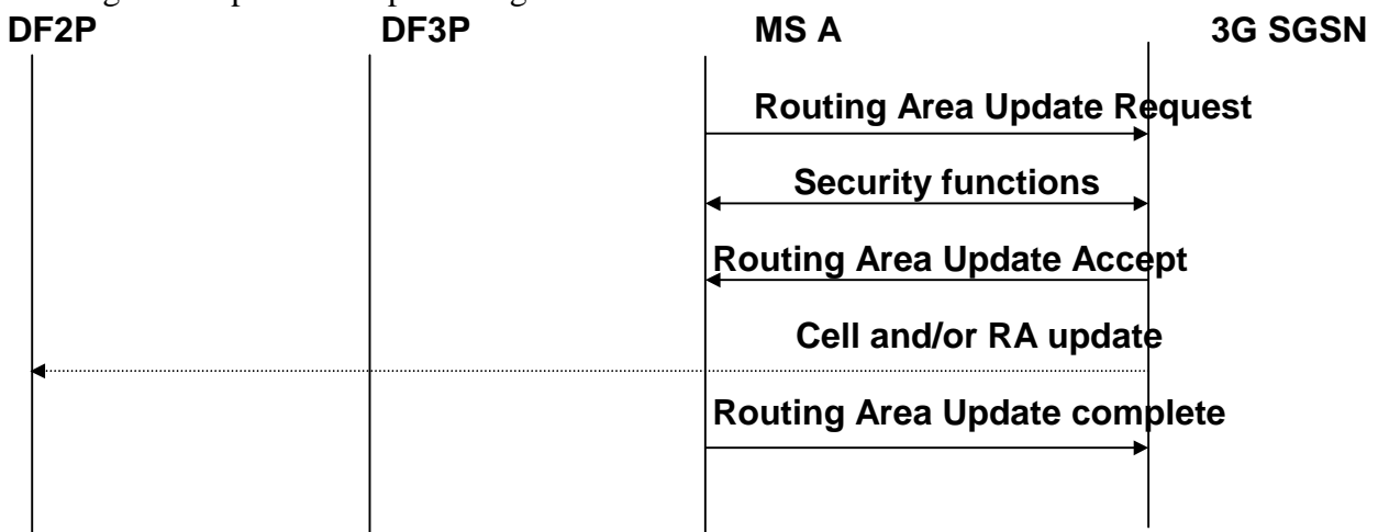
Figure B4: Interception of an Intra Routing Area Update
