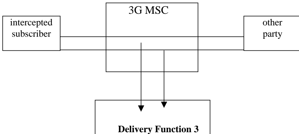
Figure 12: Bridged Access
