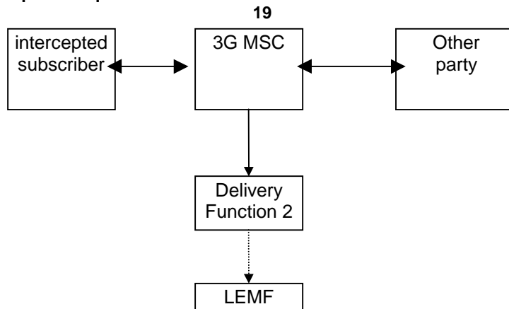
Figure 15: Provision of Intercept Related Information
