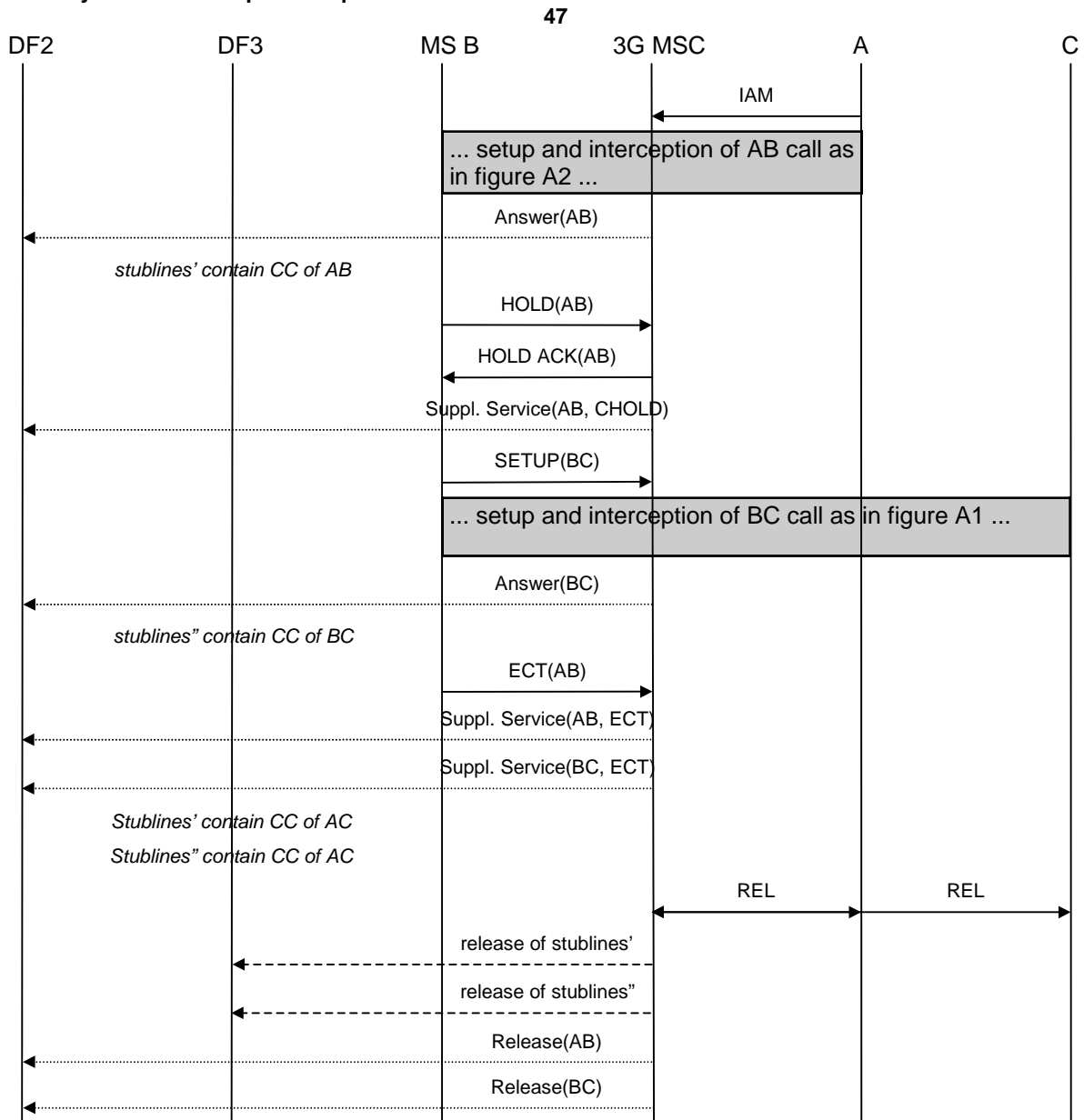
Figure A13: Interception of explicit call transfer - stublines per target call
