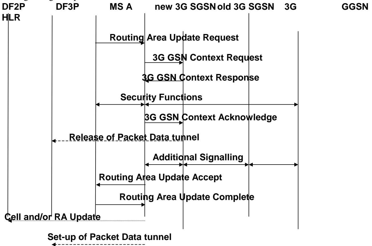
Figure B5: Interception of an Inter Routing Area Update
