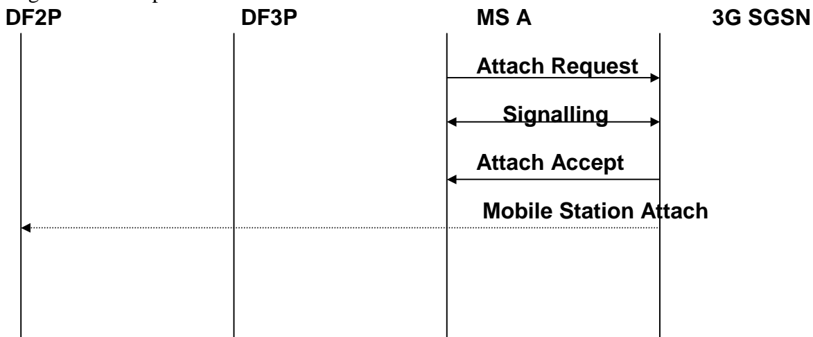
Figure B1: Interception of mobile originated Mobile Station Attachment
