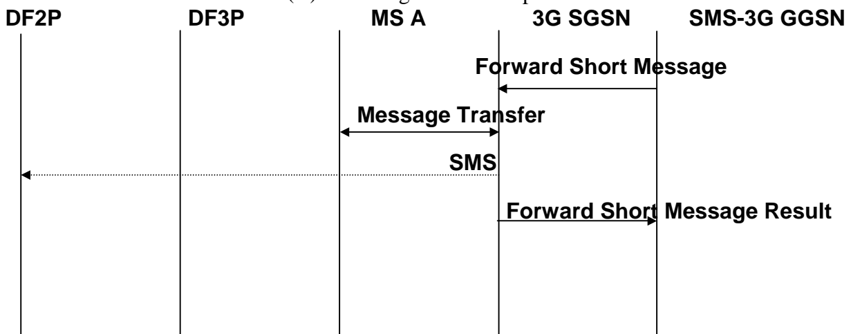
Figure B9: Interception of a Mobile-terminated SMS transfer
