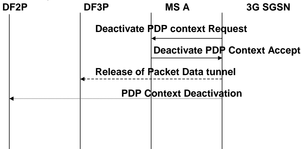
Figure B8: Interception of a Network initiated PDP Context Deactivation
