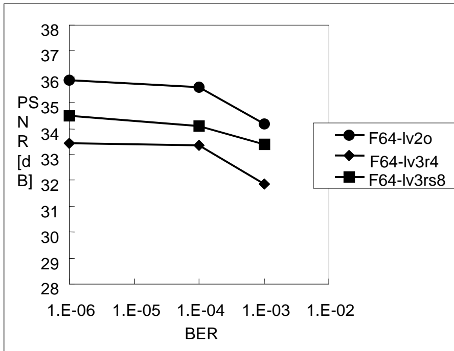
Figure 2 BER vs. PSNR performance (64 Kbit/s, Fix-to-Mobile)
