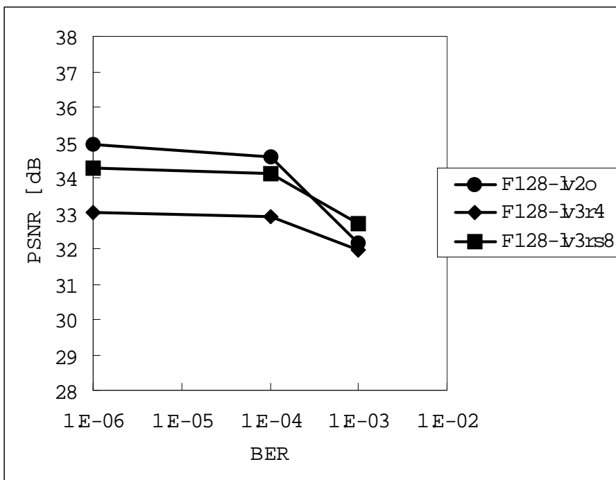
Figure 3 BER vs. PSNR performance (128 Kbit/s, Fix-to-Mobile)
