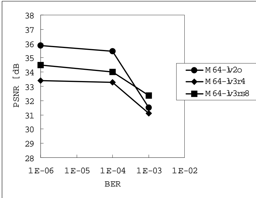
Figure 4 BER vs. PSNR performance (64 Kbit/s, Mobile-to-Mobile)
