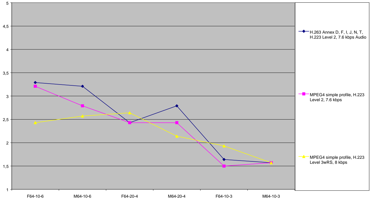
Mos versus bit-error-rate, 64kps, Australia
