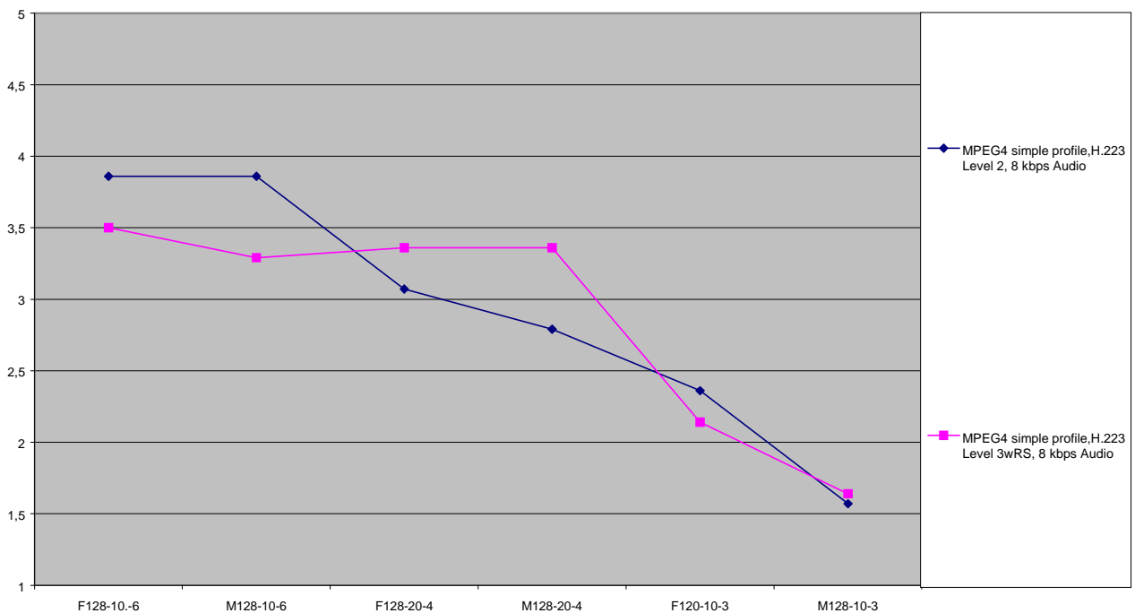
MOS versus bit-error-rate, 128 kps, Australia
