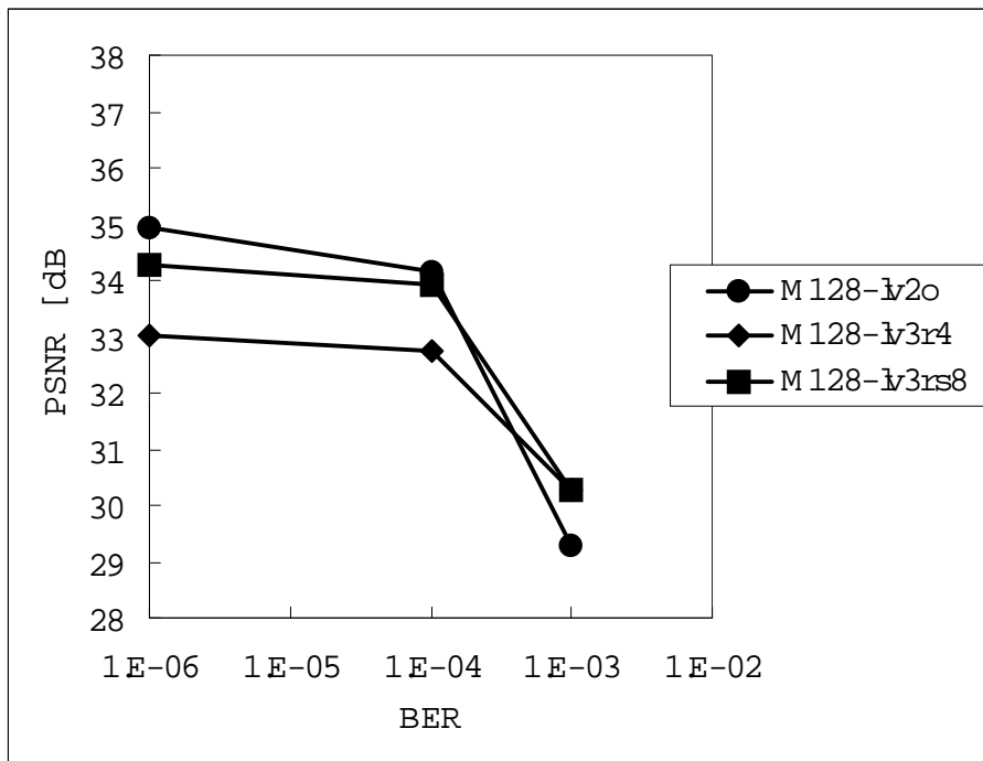
Figure 5 BER vs. PSNR performance (128 Kbit/s, Mobile-to-Mobile)
