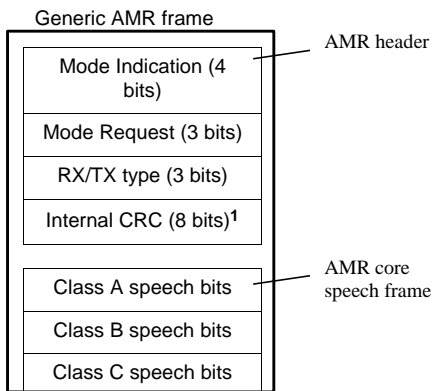
Figure 1. General frame structure
