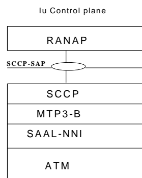
Figure 1 SAP between RANAP and its transport for Iu CS Domain
