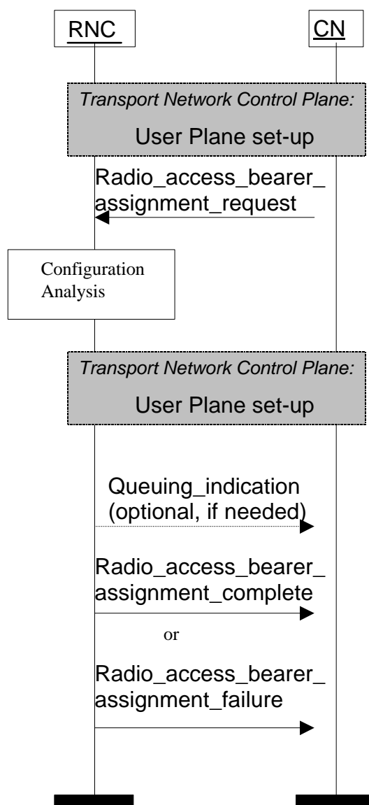
Figure 355. Radio Access Bearer Assignment procedure.
