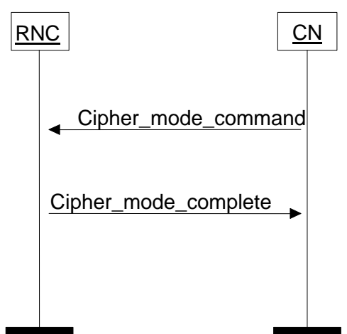
Figure 141613 . Cipher Mode Control procedure, successful case.
