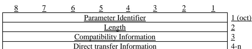
Figure 9.2.4.2-13 format of Direct transfer Information
