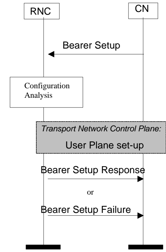
Figure 4. Bearer Setup procedure.
