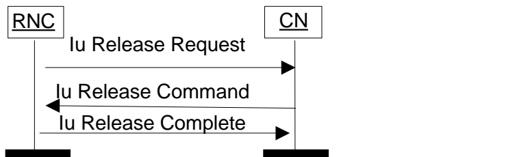
Figure 57. Iu Release: UTRAN generated reasons.
