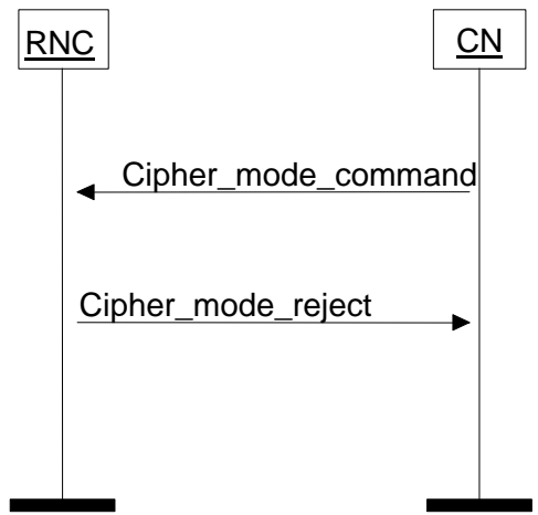
Figure 151714. Cipher Mode Control procedure, unsuccessful case.
