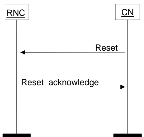
Figure 10129 . Reset at the CN.
