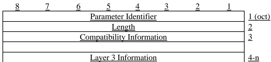
Figure 9.2.4.2-14 format of Layer 3 Information
