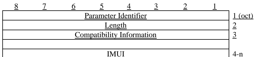
Figure 9.2.4.2-15 format of IMUI
