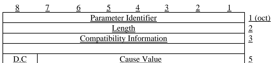
Figure 9.2.4.2-10 format of Cause
