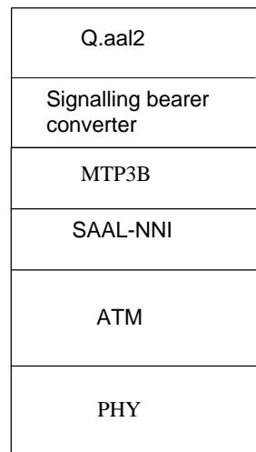
Figure 1924. Signalling bearer for Q.aal2 on Iu.
