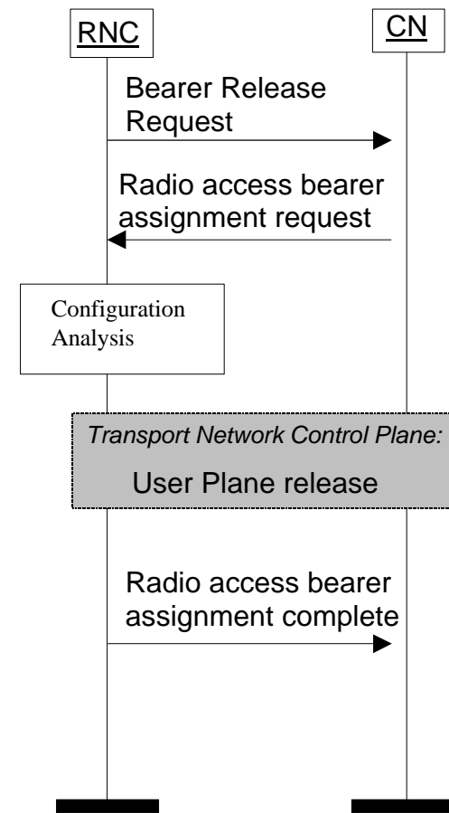
Figure 244. Radio Access Bearer Assignment procedure, UTRAN generated release.
