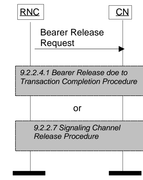
Figure 6. Bearer Release procedure, UTRAN generated release
