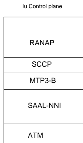
Figure 182017. Iu Signalling bearer of RANAP.
