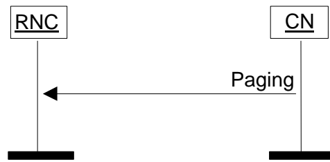
Figure 121411 . Paging procedure.
