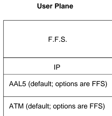
Figure 2022. Iu user plane protocol stack for the packet domain.
