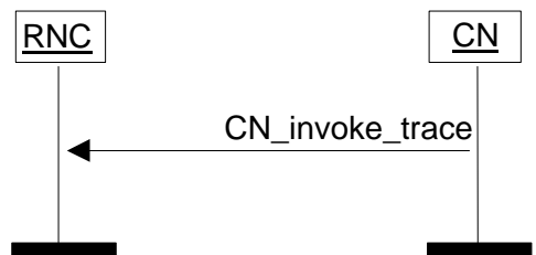
Figure 131512 . Trace Invocation procedure.
