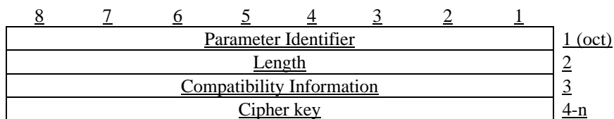
Figure 9.2.4.2-17 format of Cipher Information
