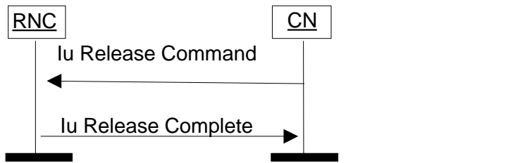
Figure 46. Iu Release: Completion of transaction between UE and CN.
