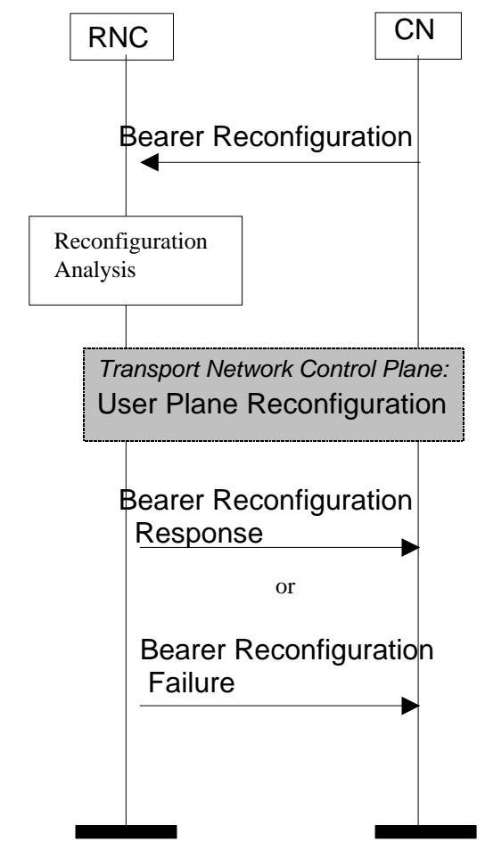
Figure 7. Bearer Reconfiguration procedure.
