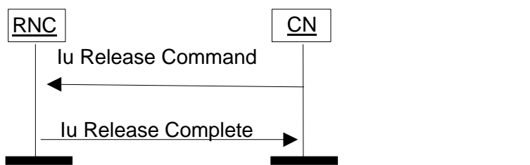
Figure 68. Iu Release: successful handover or SRNS relocation.
