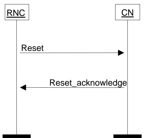
Figure 9118 . Reset at the UTRAN.
