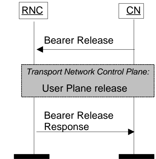
Figure 5. Bearer Release procedure
