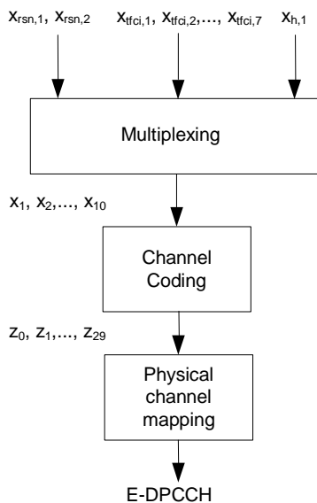
Figure 9.3.1: Coding chain for E-DPCCH
