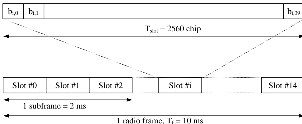
Figure 8.2.1: E-HICH/E-RGCH structure
