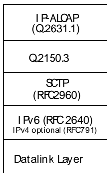
Figure B.1. Protocol stack for IP-ALCAP in IP-ATM interworking alternative 2
