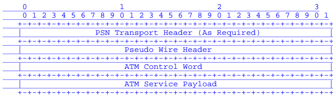
Figure 2: General format for ATM encapsulation over PSNs
