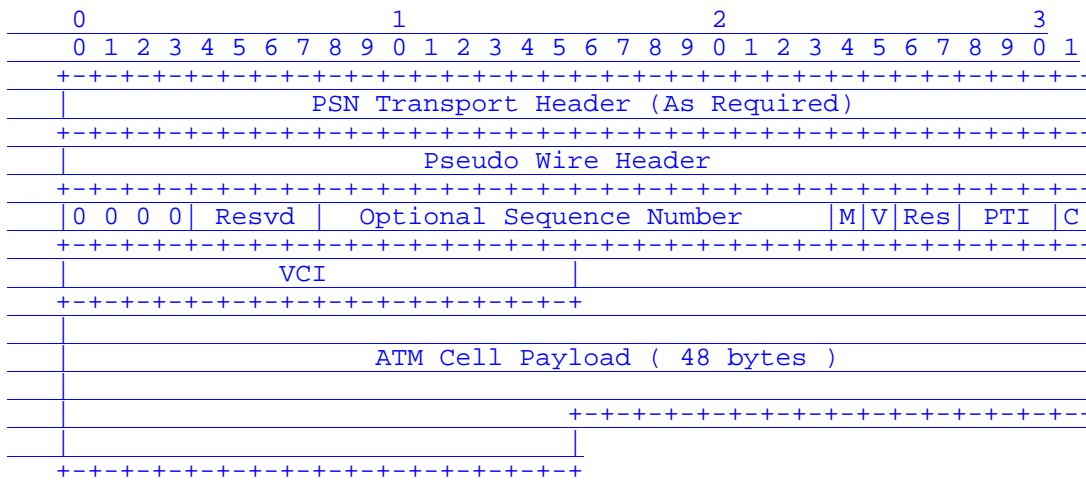
Figure 9: Single Cell VPC Encapsulation
