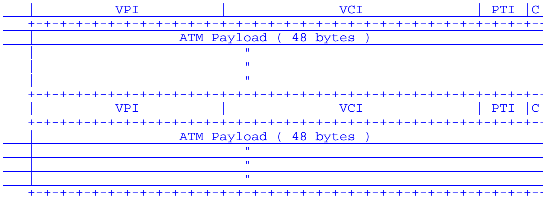
Figure 5: Multiple Cell ATM Encapsulation
