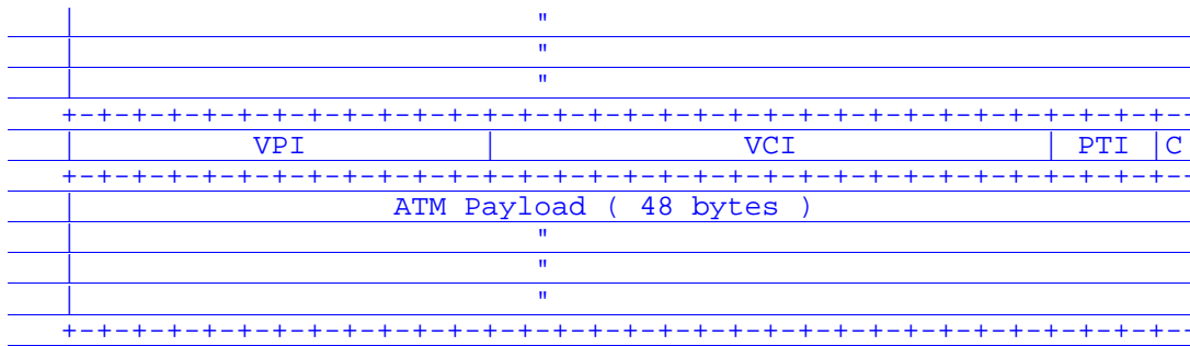
Figure 5: Multiple Cell ATM Encapsulation
