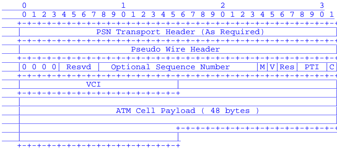
Figure 9: Single Cell VPC Encapsulation
