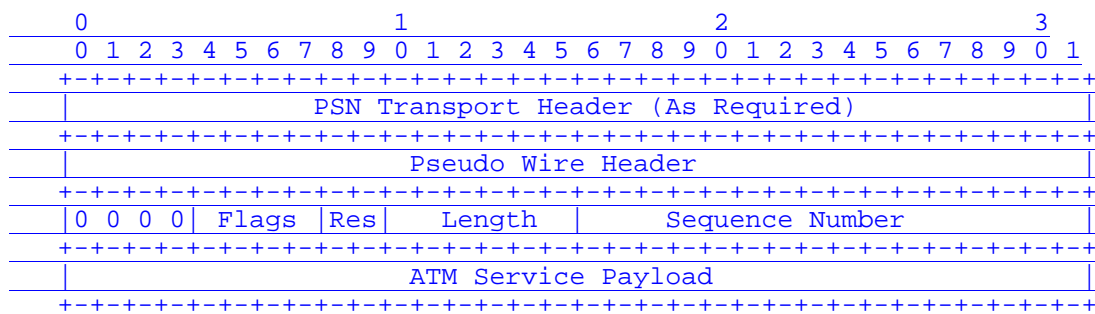
Figure 4: General format for ATM encapsulation over PSNs
