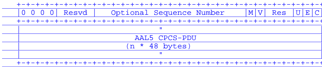
Figure 12: AAL5 transparent service encapsulation
