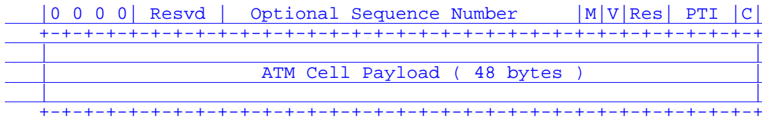
Figure 7: Single ATM VCC Cell Encapsulation
