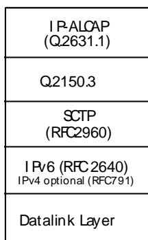
Figure B.1. Protocol stack for IP-ALCAP in IP-ATM interworking alternative 2
