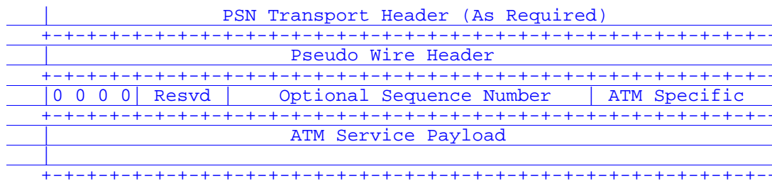
Figure 6: General format for One-to-one mode encapsulation over PSNs
