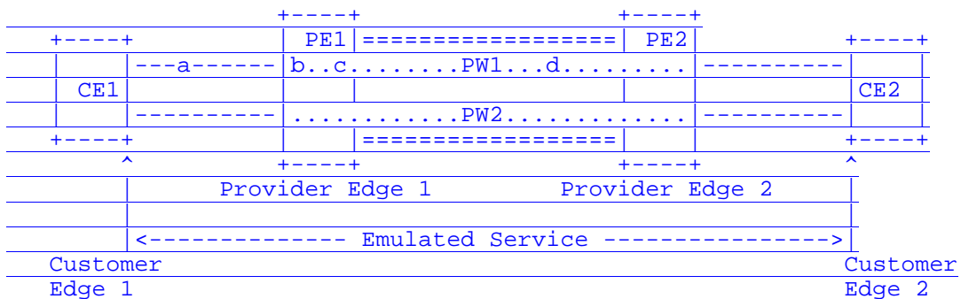
Figure 3: Defect Locations
