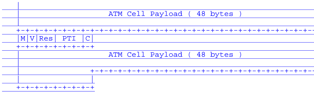
Figure 8: Multiple ATM VCC Cell Encapsulation
