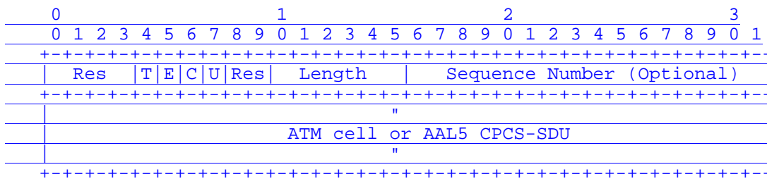
Figure 11: AAL5 CPCS-SDU Encapsulation
