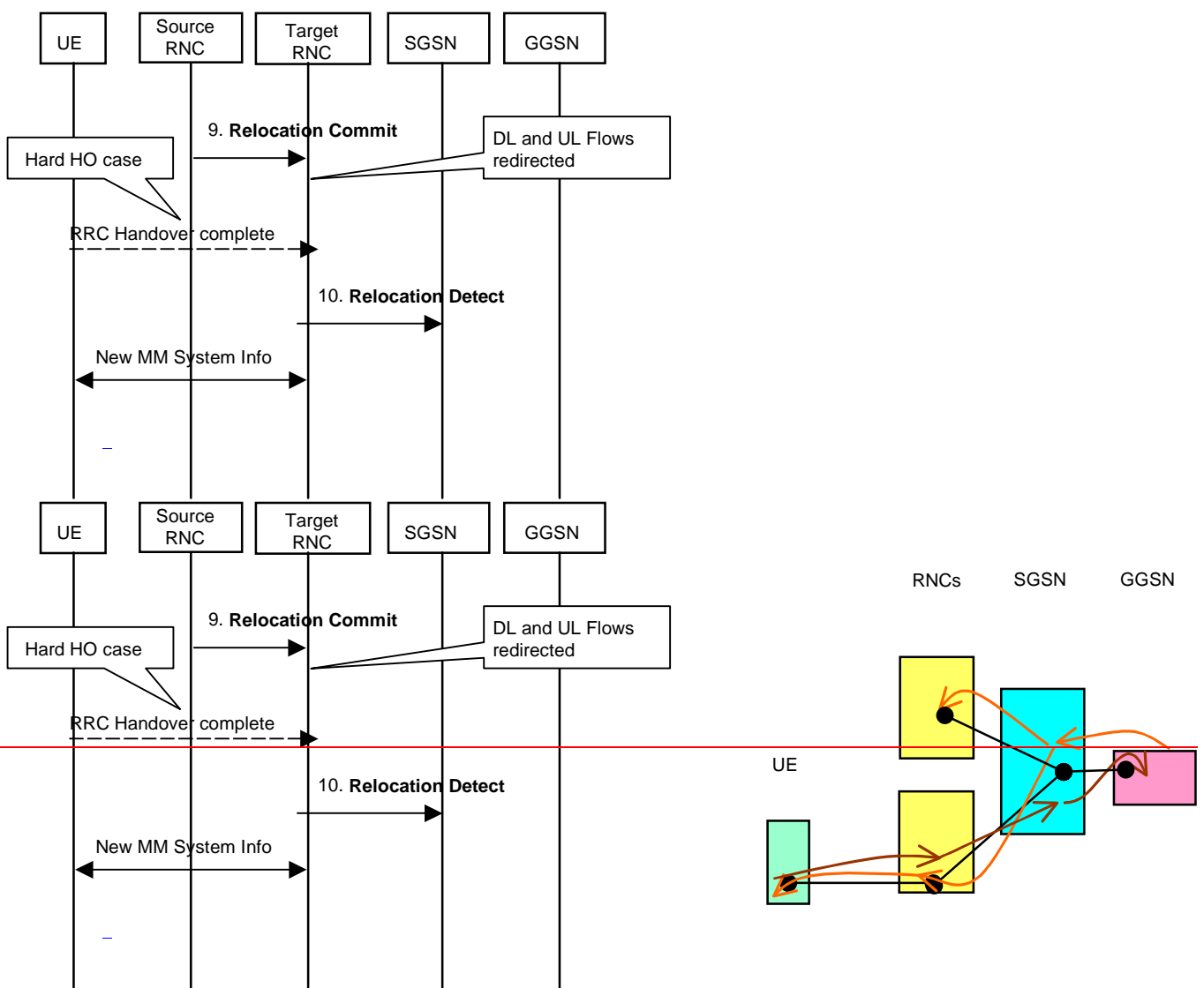
Figure 23: Control Plane - Bi-casting of DL flow and switching of UL flow phase with only one SGSN
