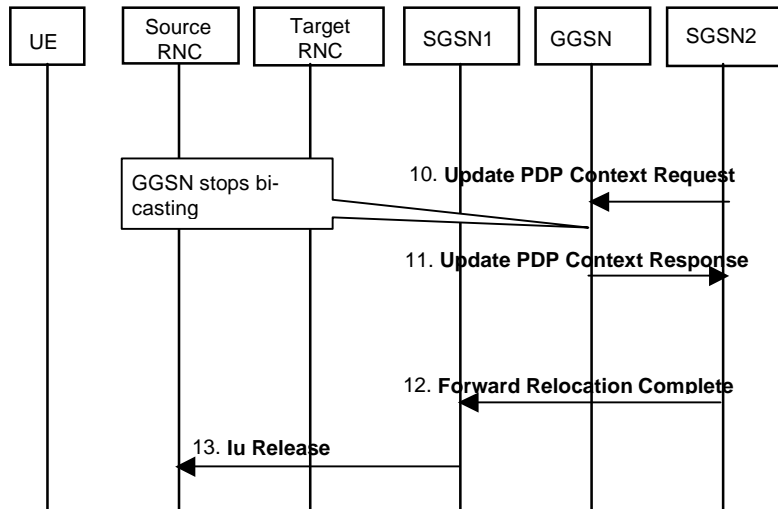
Figure 17: Control Plane – Completion with 2 SGSNs involved
