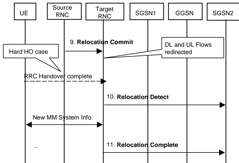
Figure 14 : Control Plane - Bi-casting of DL flow and switching of UL flow phase with 2 SGSNs involved
