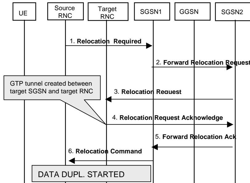
Figure 1 : Control Plane - Preparation of Relocation of SRNS and Resource allocation phase
