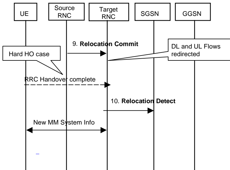
Figure 23: Control Plane - Bi-casting of DL flow and switching of UL flow phase with only one SGSN
