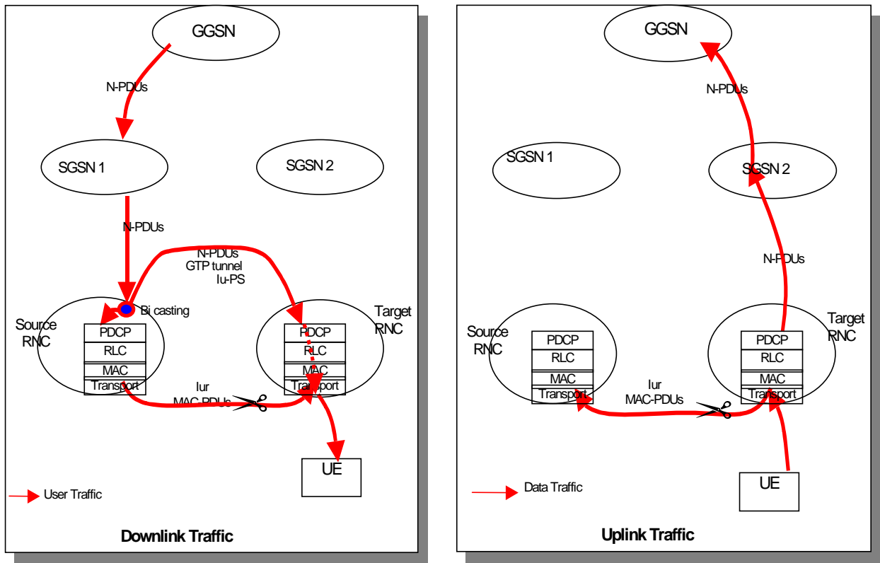
Figure 5 : User Plane - Moving the Serving RNC role to target RNC ( SRNS Relocation)
