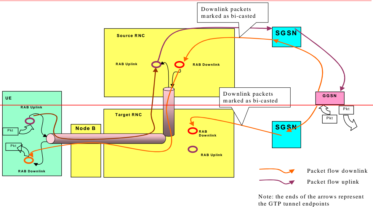
Figure 102: Packet flows during relocation, solution 2
