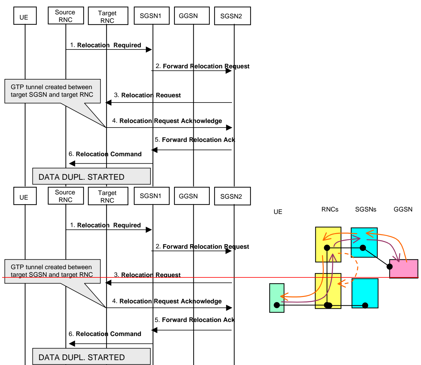
Figure 1 : Control Plane - Preparation of Relocation of SRNS and Resource allocation phase
