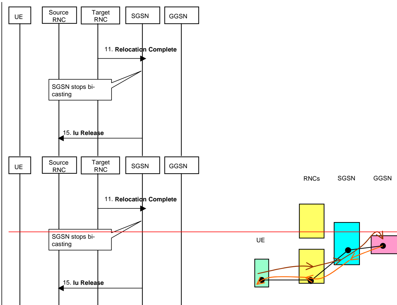
Figure 26: Control Plane – Completion phase with only one SGSN
