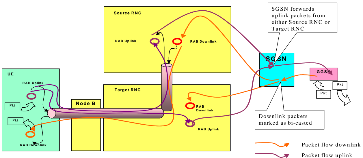
Figure 319: Packet flows during relocation with only one SGSN involved, solution 2
