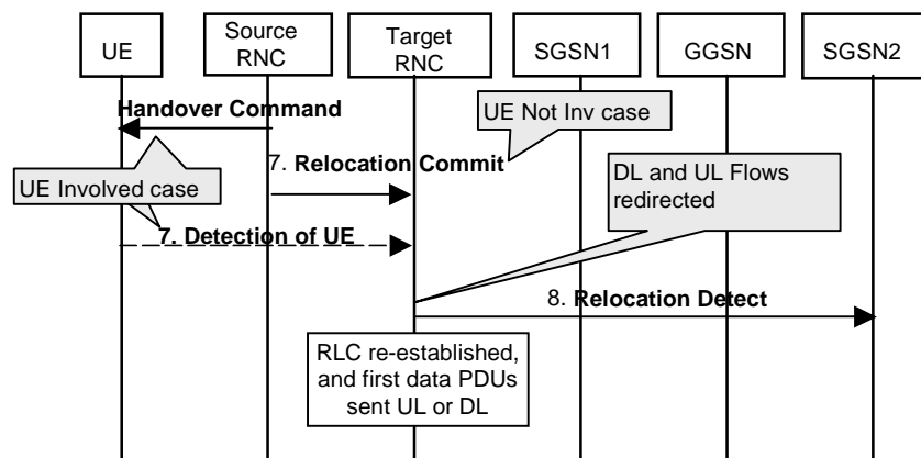
Figure 4 : Control Plane - Moving the Serving RNC role to target RNC
