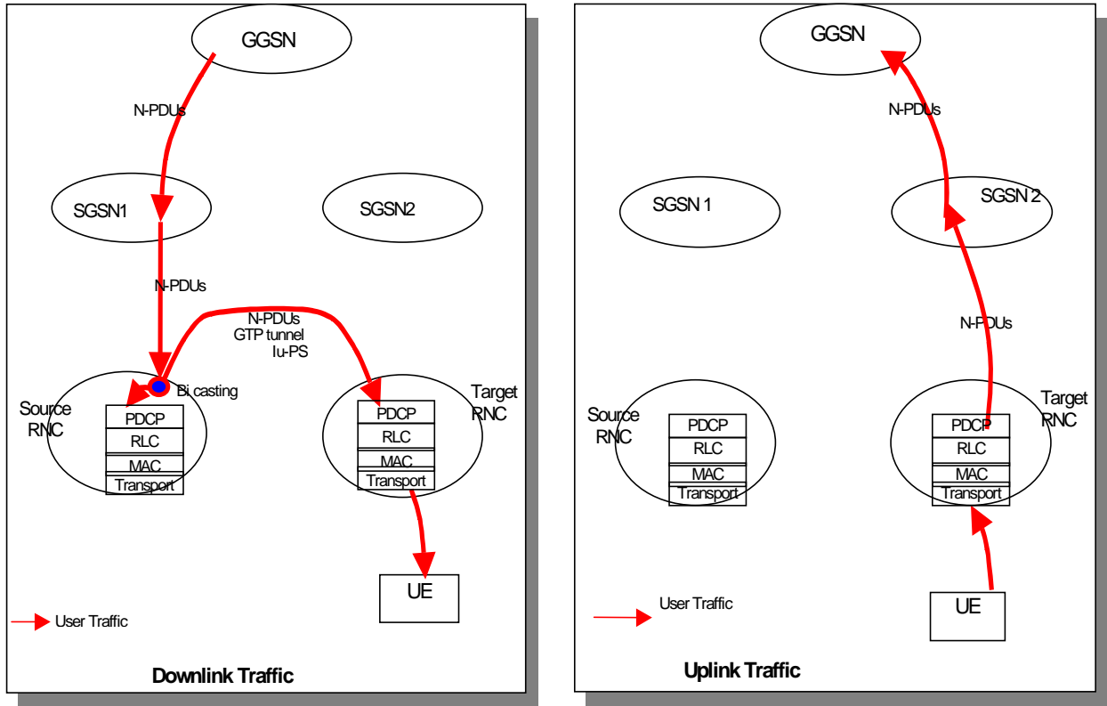
Figure 6 : User Plane - Moving the Serving RNC role to target RNC ( Hard Handover)
