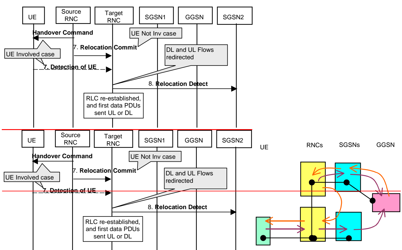
Figure 4 : Control Plane - Moving the Serving RNC role to target RNC
