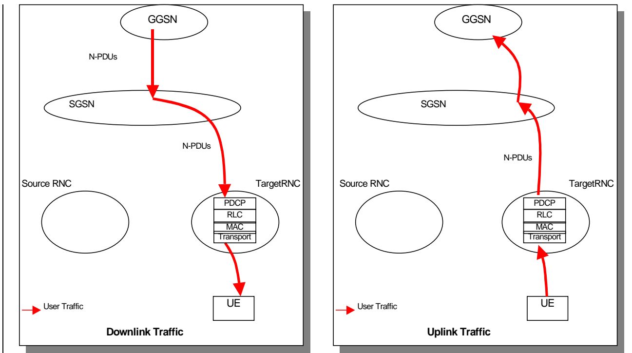
Figure 27: User Plane – Completion phase with only one SGSN
