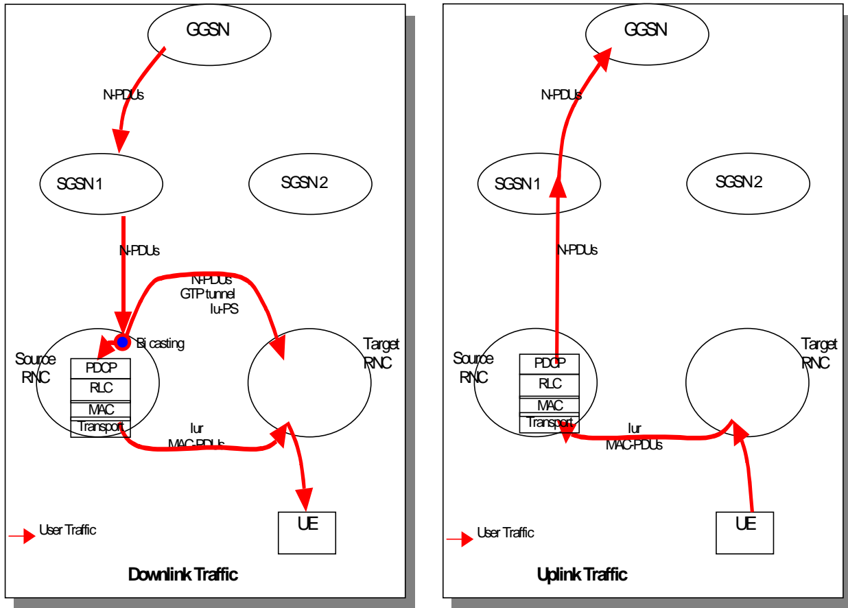
Figure 2 : User Plane - Preparation of Relocation of SRNS and Resource allocation (SRNS Relocation)
