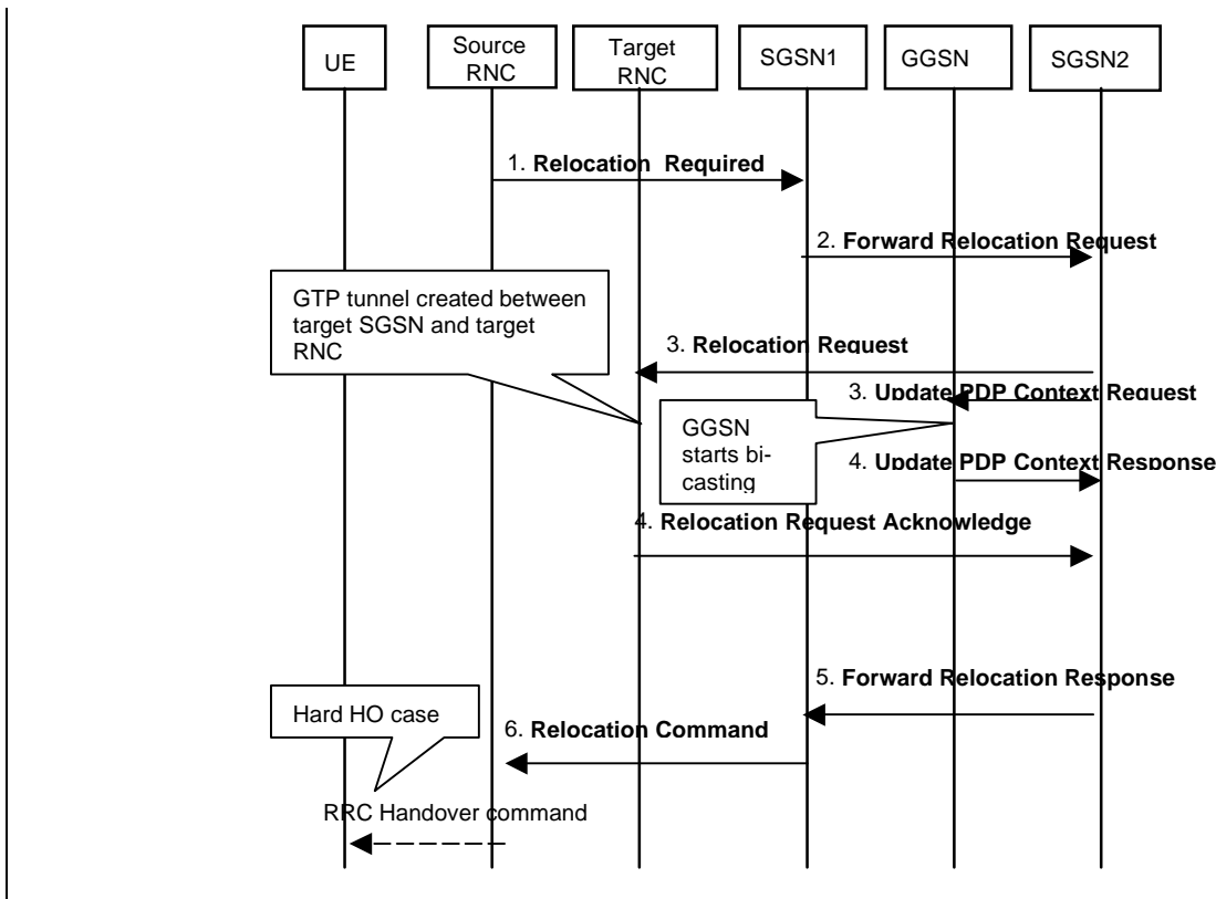
Figure 9 : Control Plane – Preparation involving 2 SGSNs
