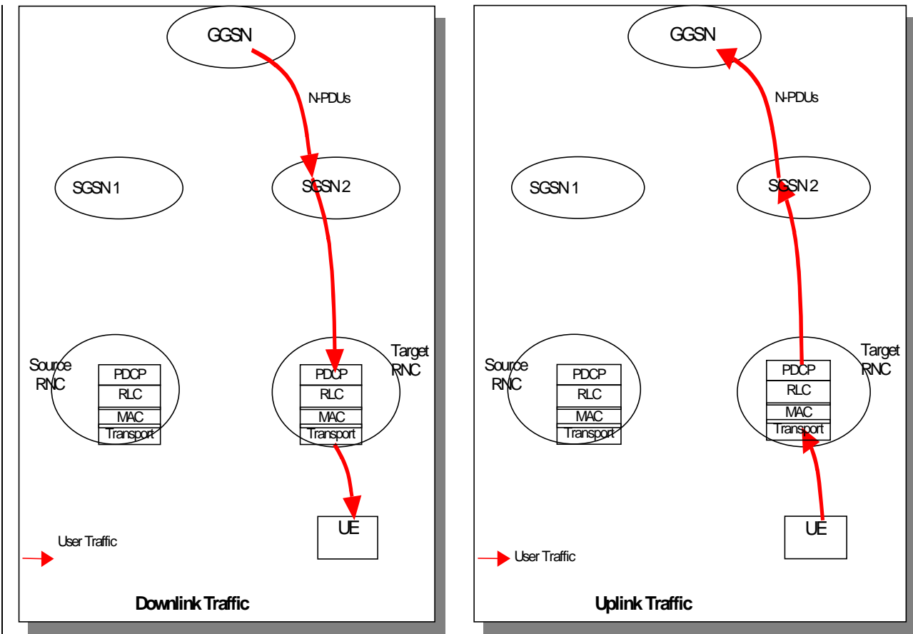
Figure 8 : User Plane - Switching of DL flow in CN
