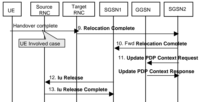
Figure 7 : Control Plane - Switching of DL flow in CN phase
