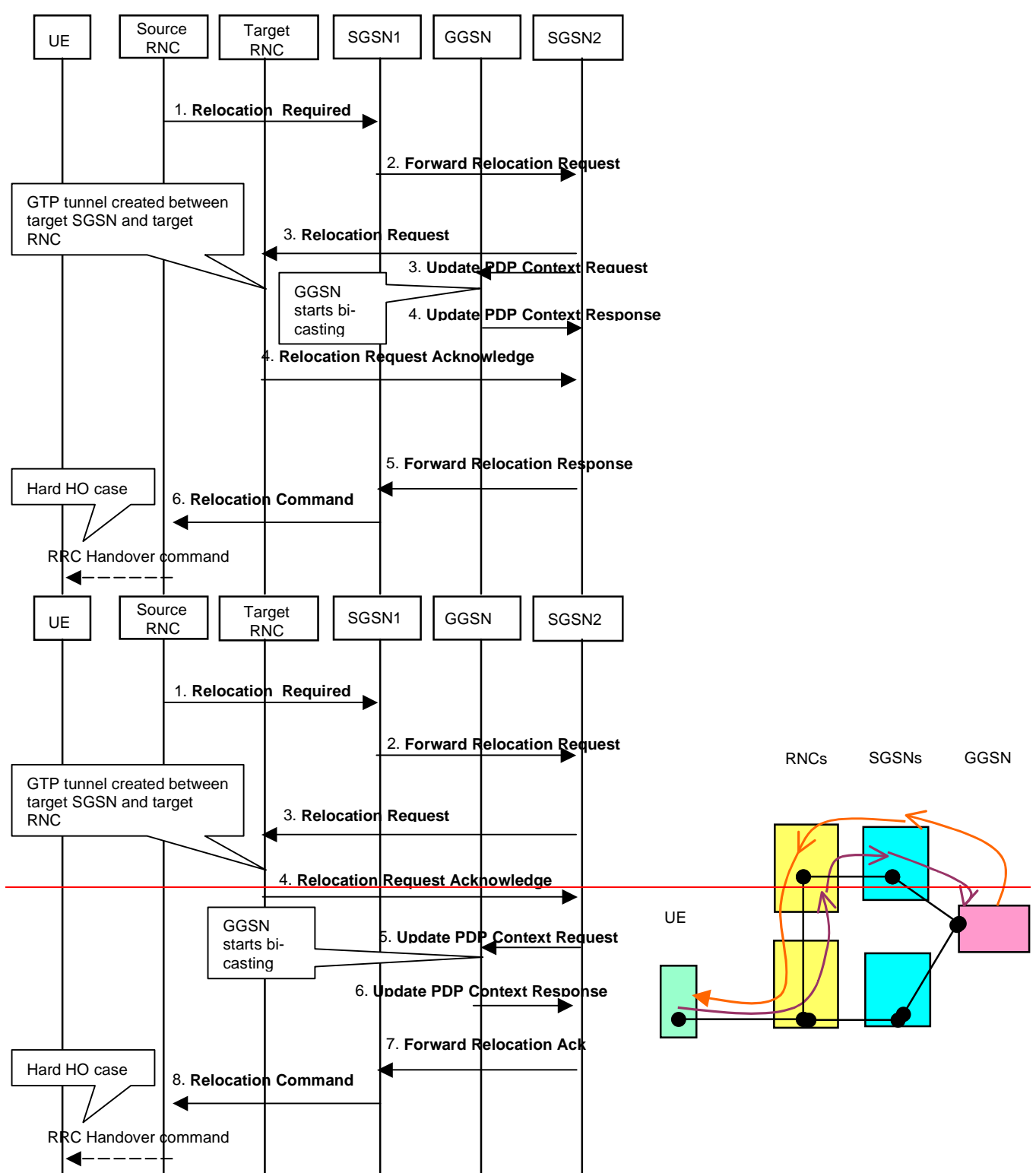
Figure 9 : Control Plane – Preparation involving 2 SGSNs
