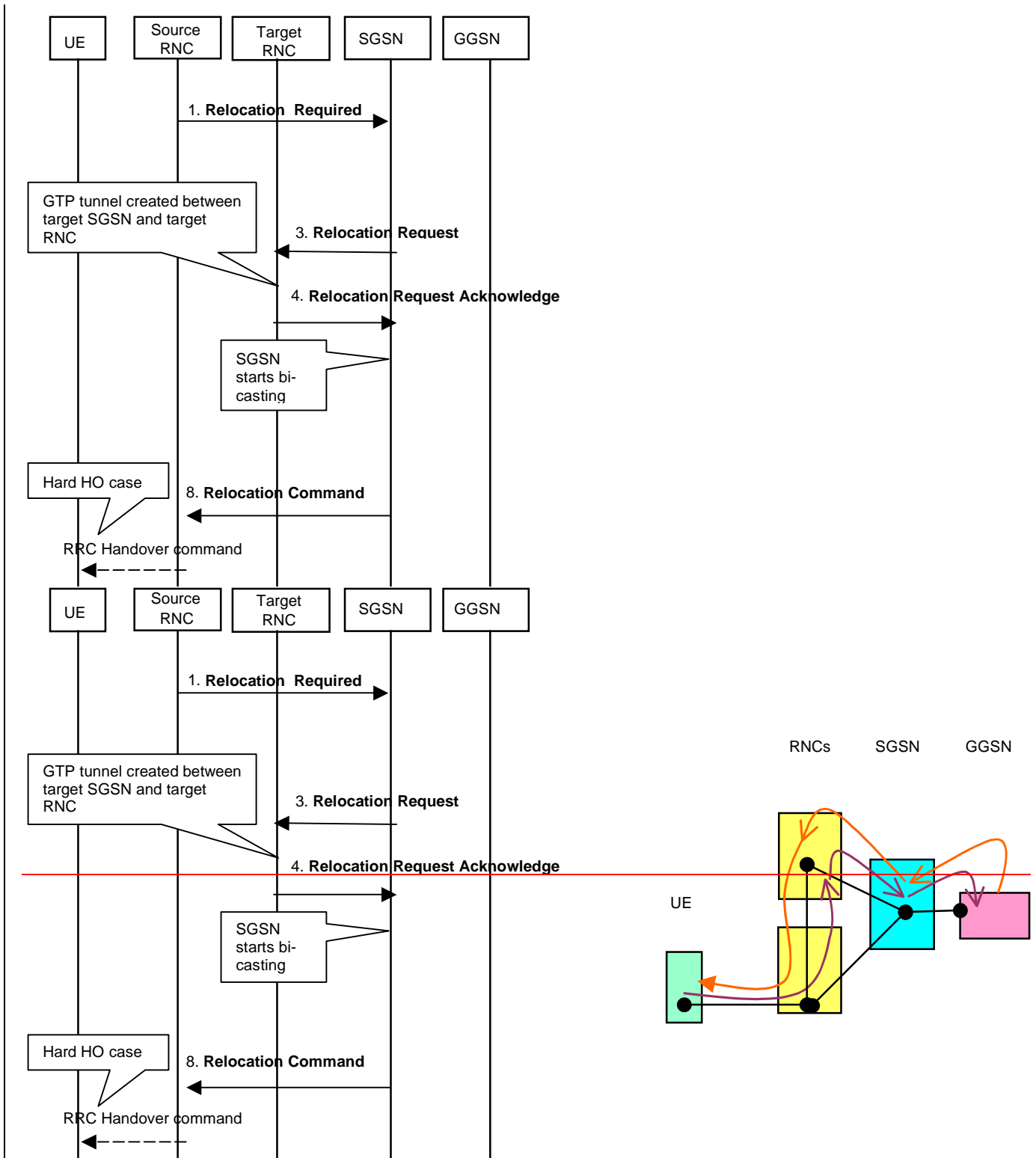
Figure 20: Control Plane – Preparation phase with only one SGSN
