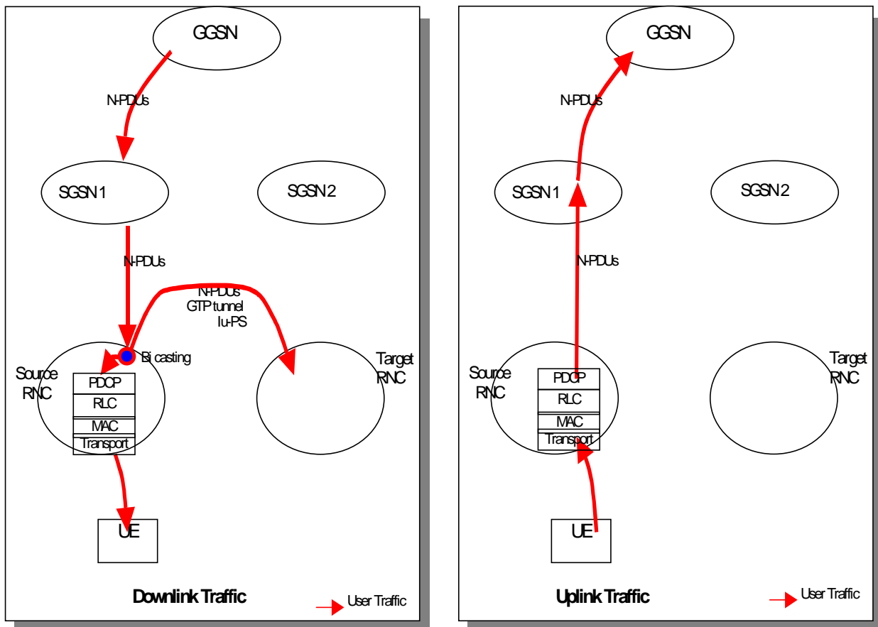
Figure 3 : User Plane - Preparation of Relocation of SRNS and Resource allocation (Hard Handover)
