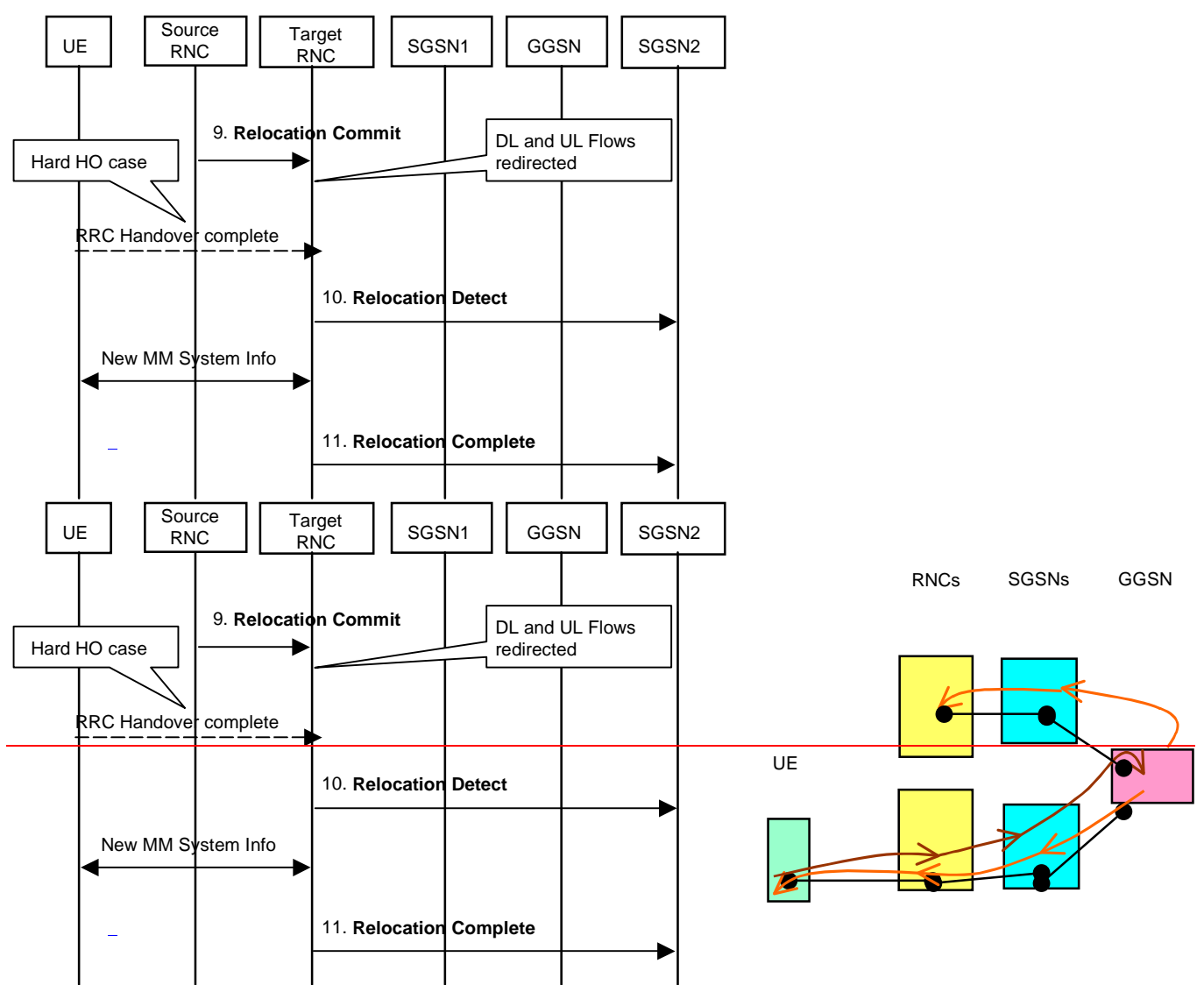
Figure 14 : Control Plane - Bi-casting of DL flow and switching of UL flow phase with 2 SGSNs involved
