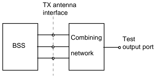
Figure 5.142.5.2: Transmitter test setup
