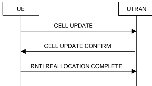
Figure 3532. Cell update procedure with RNTI reallocation
