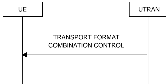
Figure 2825. Transport format combination control, normal flow
