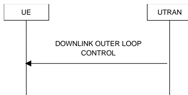
Figure 3330) Downlink Outer Loop Control , normal flow
