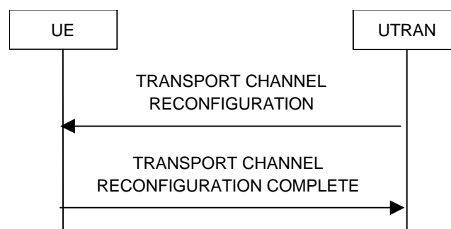
Figure 2623. Transport channel reconfiguration, normal flow
