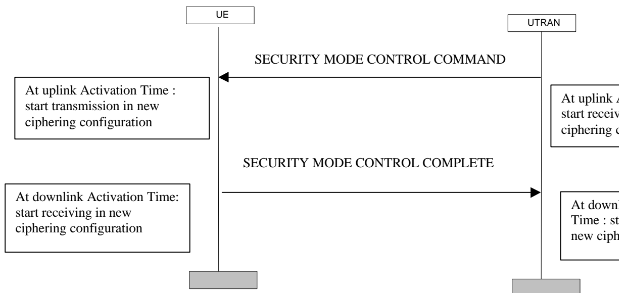
Figure 1916) Security mode control procedure
