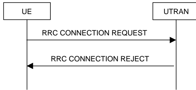
Figure 107) RRC Connection Establishment, network rejects RRC connection
