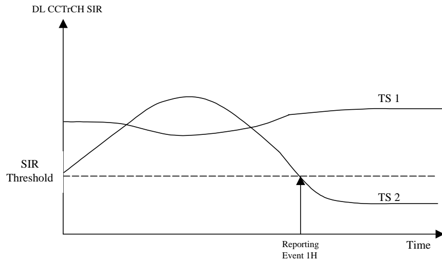
Figure 5792 A SIR value of a timeslot becomes worse than an absolute threshold
