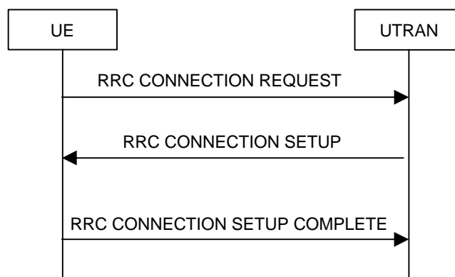
Figure 96) RRC Connection Establishment, network accepts RRC connection
