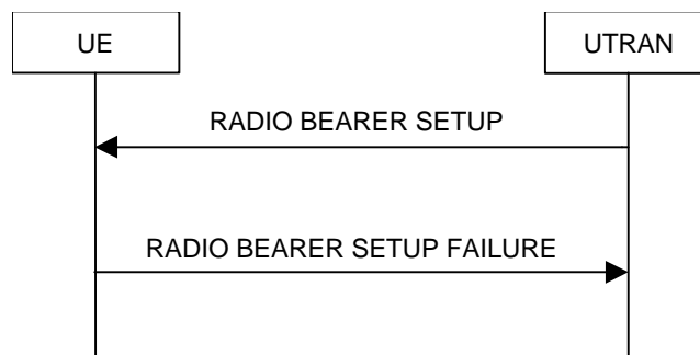
Figure 2118. Radio Bearer Establishment, UE reverts to old configuration
