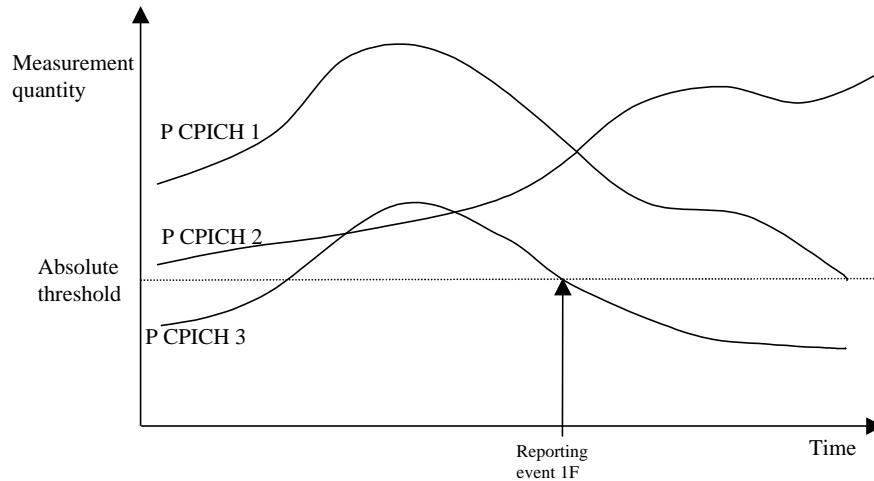
Figure 5590 Event-triggered report when a Primary CPICH becomes worse than an absolute threshold.
