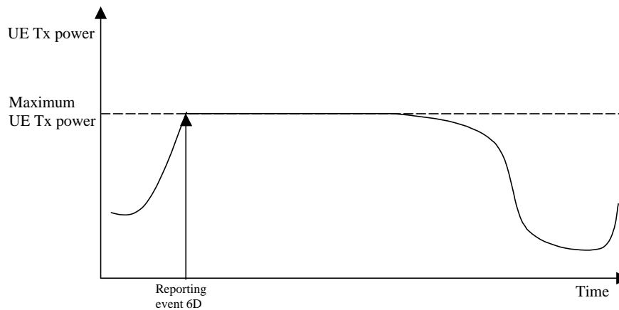
Figure 79108 Event-triggered report when the UE Tx power reaches its maximum value.
