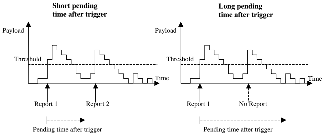
Figure 76105 Pending time after trigger limits the amount of consecutive measurement reports.
