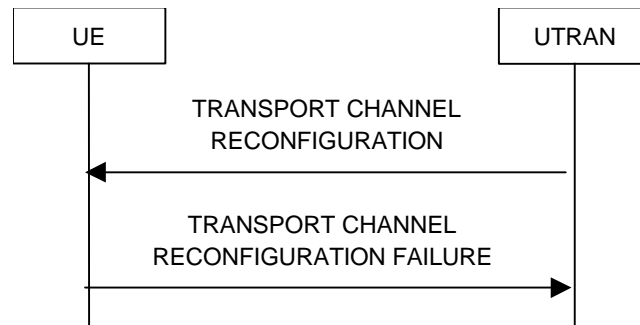
Figure 2724. Transport channel reconfiguration, failure case
