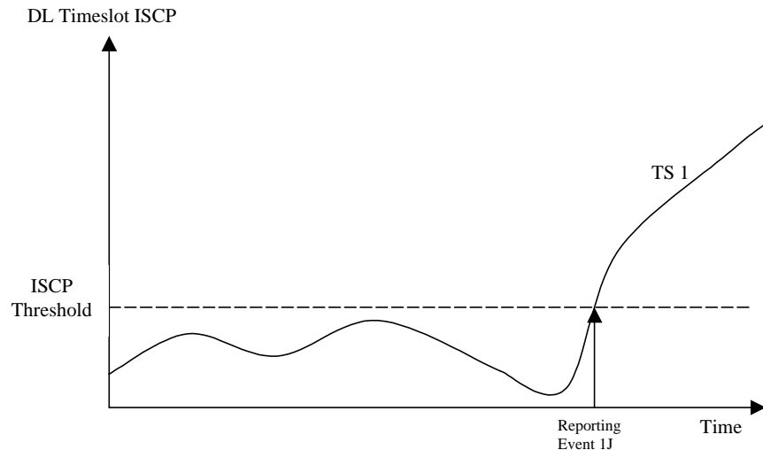
Figure 5994 A ISCP value of a timeslot becomes better than a certain threshold
