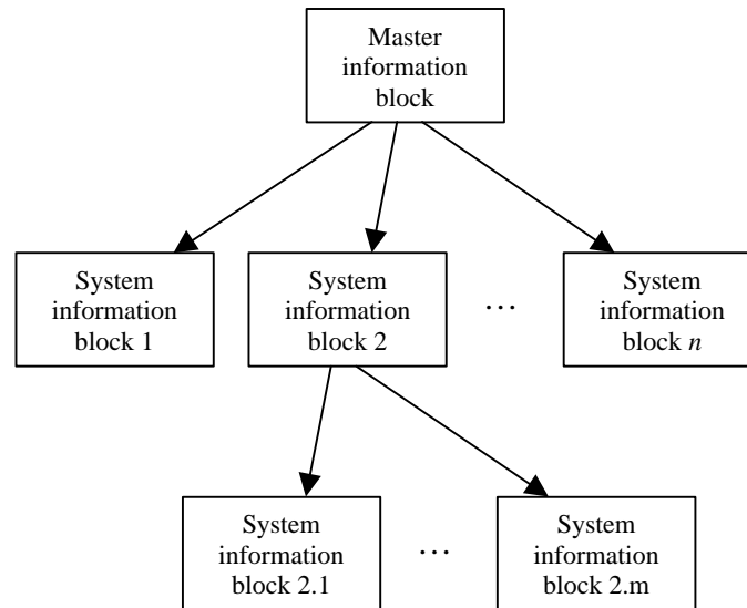
Figure 64. The overall structure of system information.
