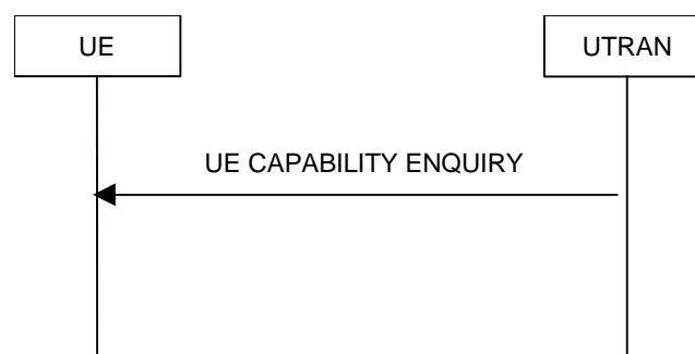
Figure 1512. UE capability enquiry procedure, normal flow
