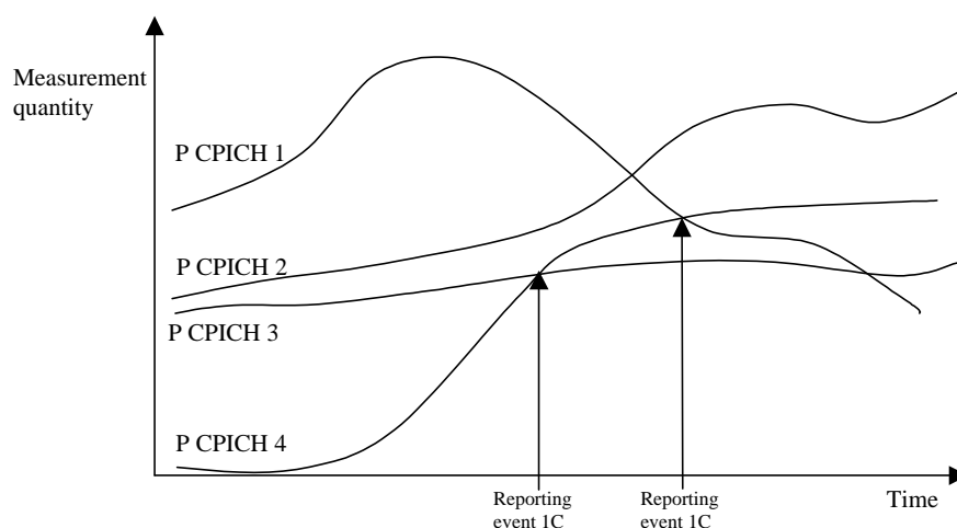
Figure 5287 A primary CPICH that is not included in the active set becomes better than a primary CPICH that is in the active set.
