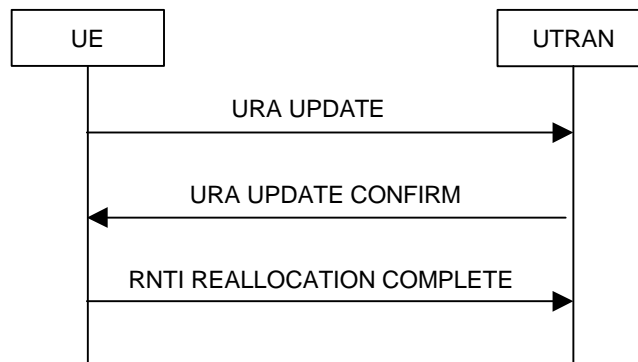
Figure 3835. URA update procedure with RNTI reallocation
