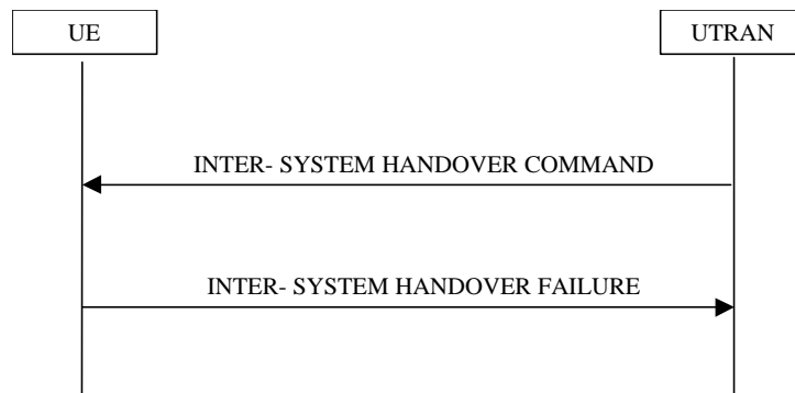
Figure 4643. Inter system handover from UTRAN, failure case
