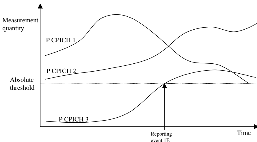
Figure 5489 Event-triggered report when a Primary CPICH becomes better than an absolute threshold.
