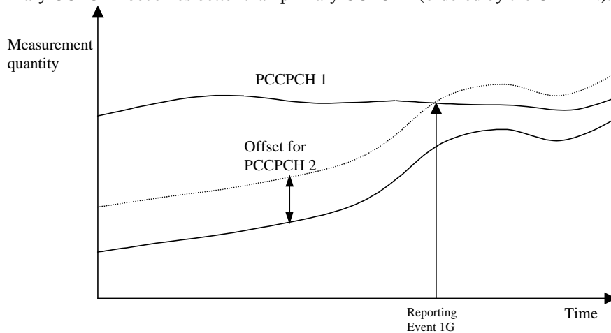
Figure 71102 A positive offset is applied to primary CCPCH 2.
