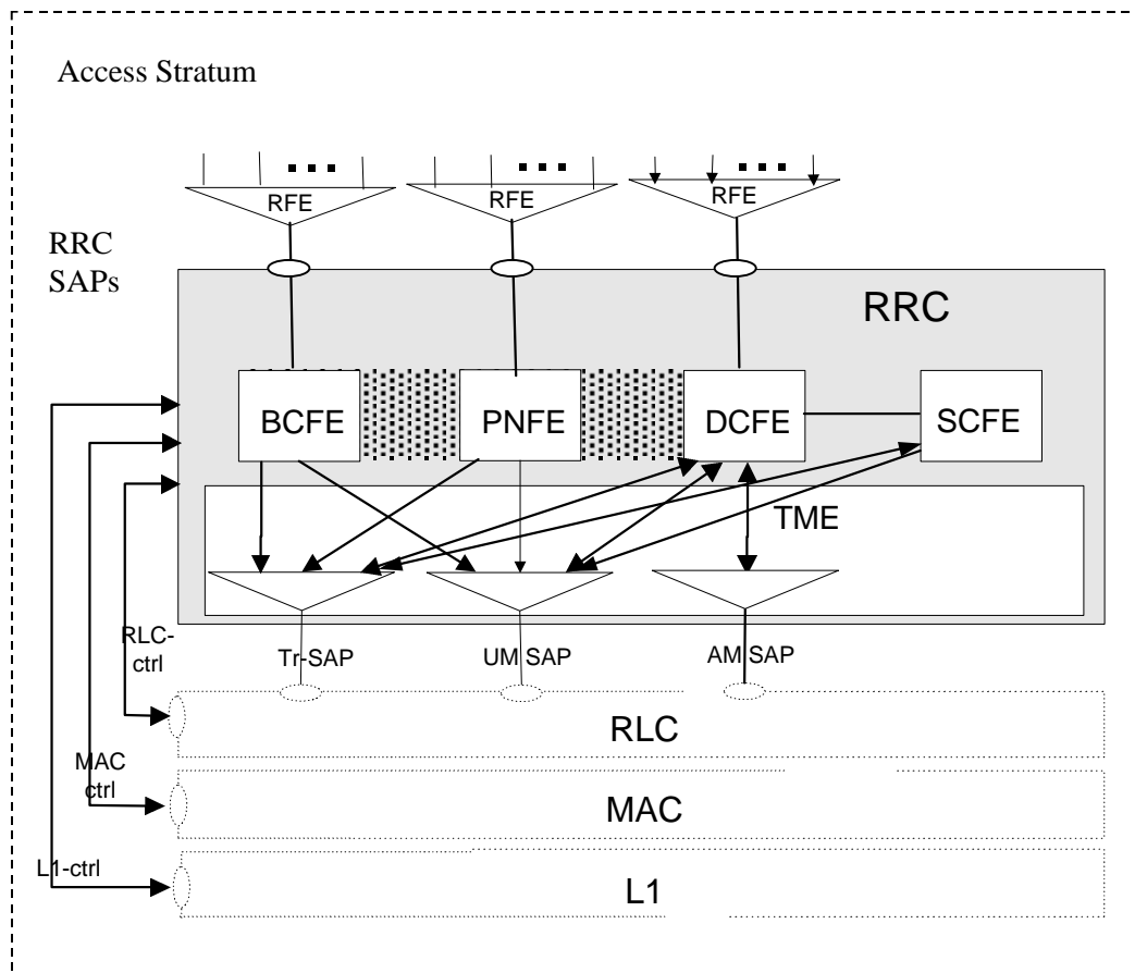
Figure 32) UTRAN side RRC model
