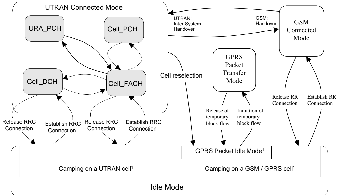
Figure 5081: RRC States and State Transitions including GSM
