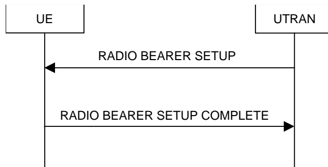
Figure 2017. Radio Bearer Establishment, normal case
