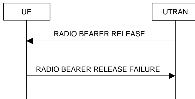
Figure 2522. Radio Bearer Release, UE reverts to old configuration
