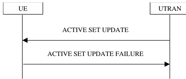
Figure 4138. Active Set Update procedure, failure case
