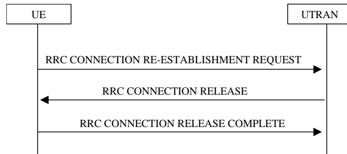
Figure 1340. RRC Connection Re-establishment, failure case
