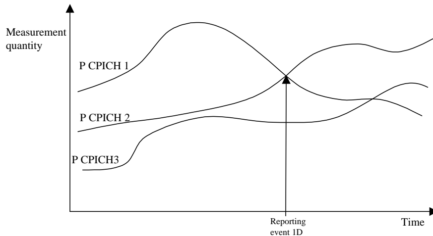
Figure 5388 A primary CPICH becomes better than the previously best primary CPICH.
