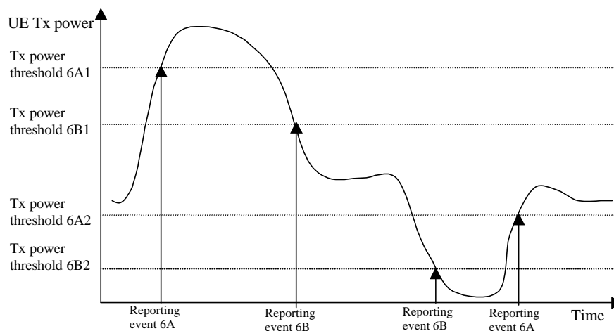
Figure 77106 Event-triggered measurement reports when the UE Tx power becomes larger or less than absolute thresholds.
