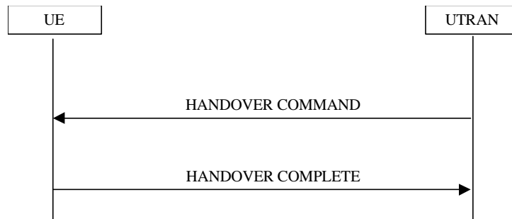
Figure 4239. Hard handover, successful case
