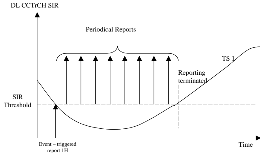
Figure 6297 Periodic reporting triggered by event 1H
