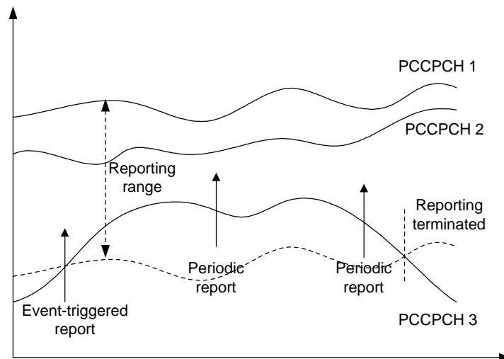
Figure 6095 Periodic reporting triggered by event 1A
