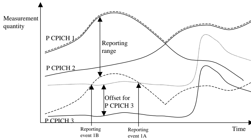
Figure 69101 A positive offset is applied to primary CPICH 3 before event evaluation in the UE.
