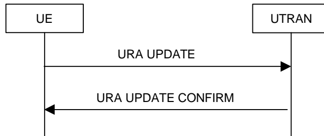
Figure 3734. URA update procedure, basic flow
