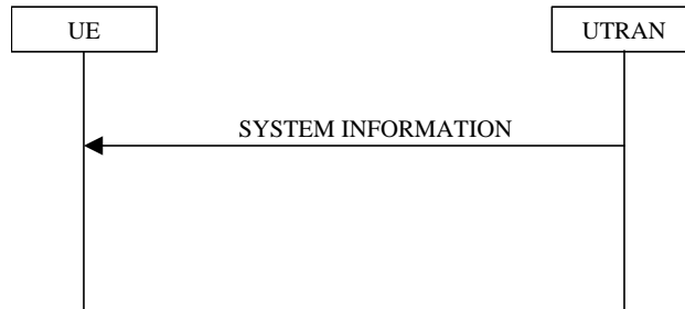
Figure 53. Broadcast of system information
