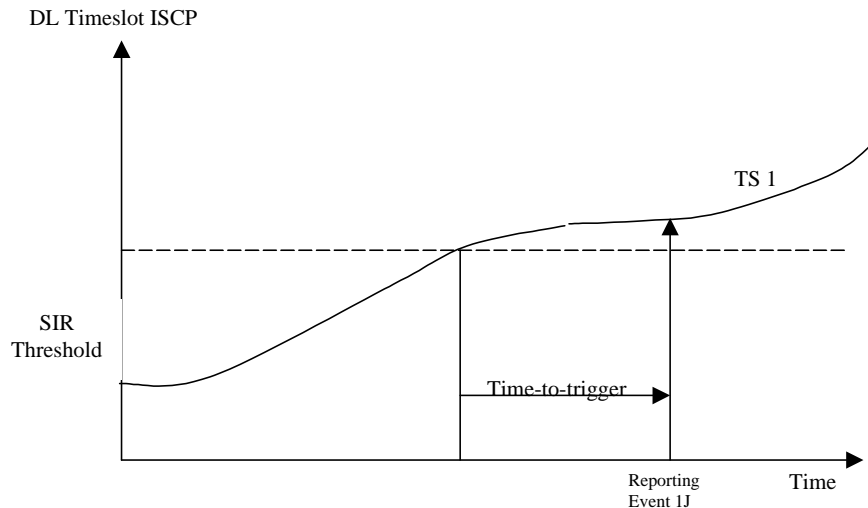
Figure 67100 Time-to-trigger limits the amount of measurement reports.
