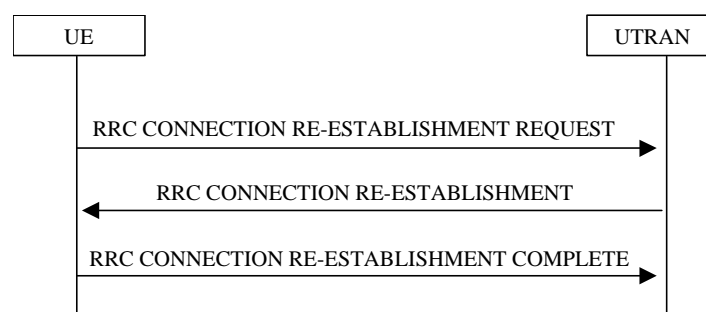
Figure 129. RRC Connection Re-establishment, successful case
