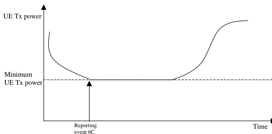
Figure 78107 Event-triggered measurement report when the UE Tx power reaches its minimum value.
