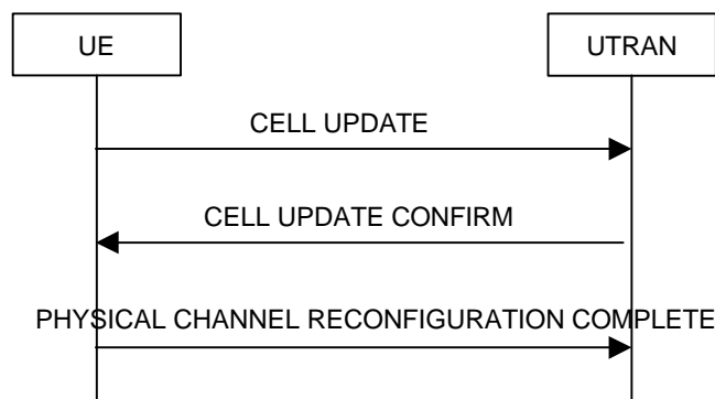
Figure 3633. Cell update procedure with physical channel reconfiguration
