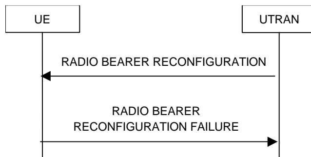
Figure 2320. Radio bearer reconfiguration, failure case
