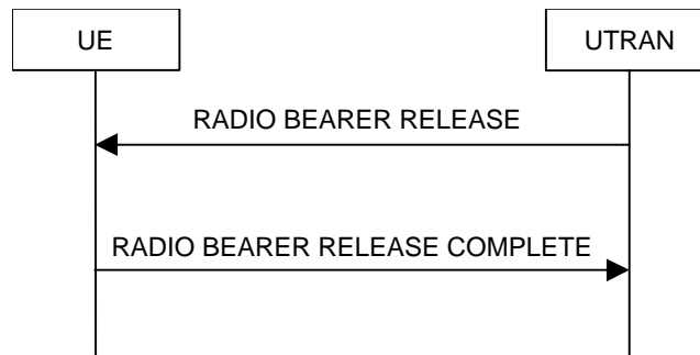
Figure 2421. Radio Bearer Release, normal case
