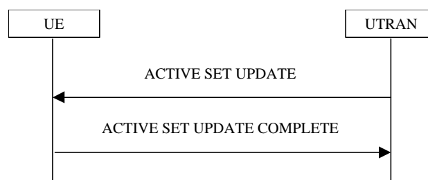
Figure 4037. Active Set Update procedure, successful case
