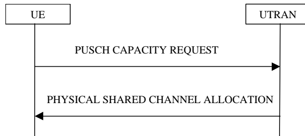
Figure 3229. PUSCH Capacity request procedure
