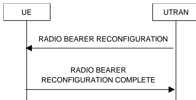
Figure 2219. Radio bearer reconfiguration, normal flow
