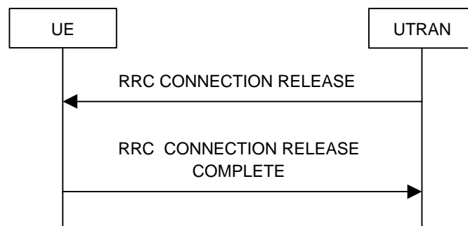
Figure 118. RRC Connection Release procedure
