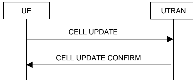
Figure 3431. Cell update procedure, basic flow
