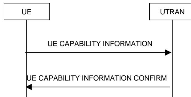
Figure 1411. Transmission of UE capability information, normal flow
