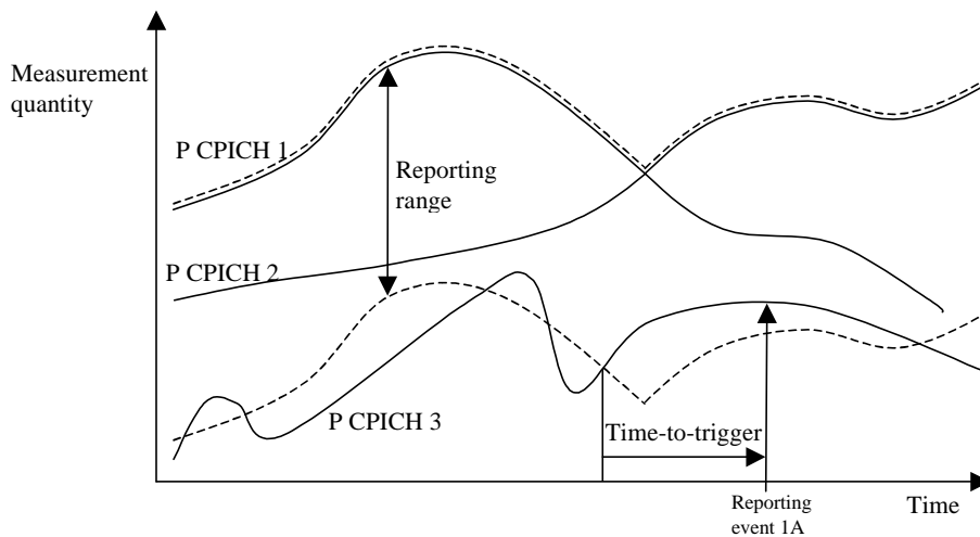
Figure 6599 Time-to-trigger limits the amount of measurement reports.
