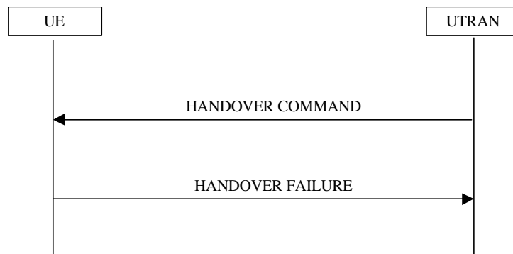
Figure 4340. Hard handover, failure case
