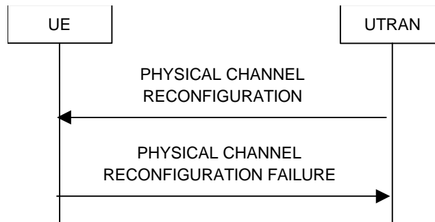
Figure 3027. Physical channel reconfiguration, failure case
