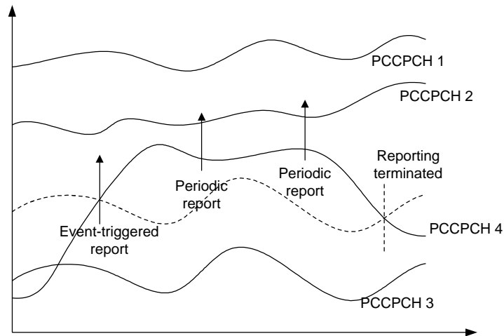
Figure 6196 Periodic reporting triggered by event 1C
