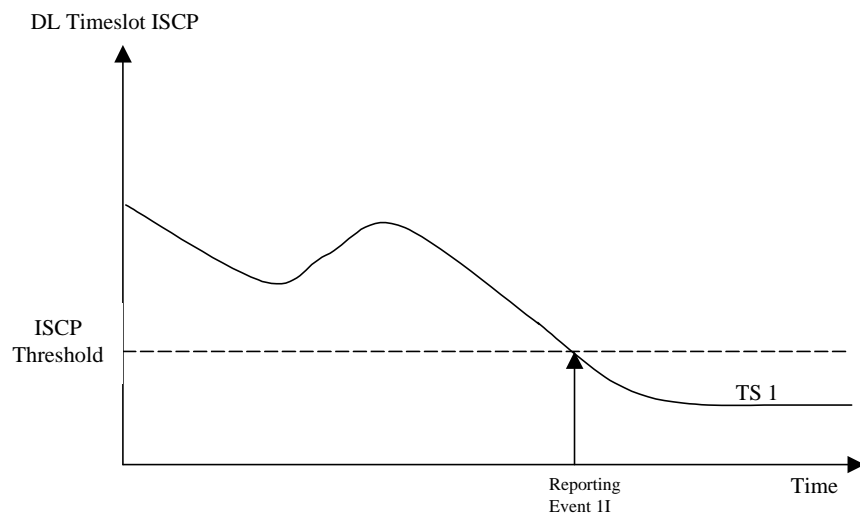
Figure 5893 A ISCP value of a timeslot becomes worse than an absolute threshold
