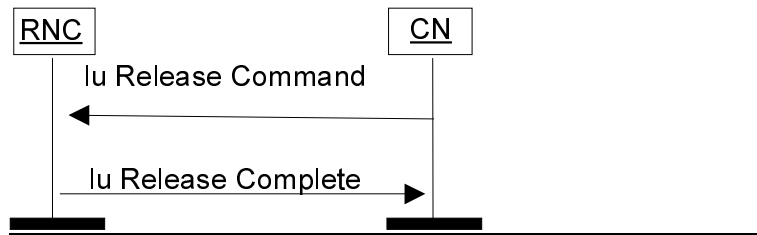
Figure 5. Iu Release: Completion of transaction between UE and CN.
