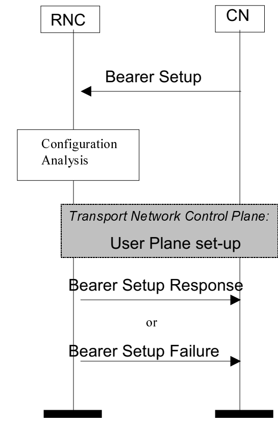
Figure 4. Bearer Setup procedure.
