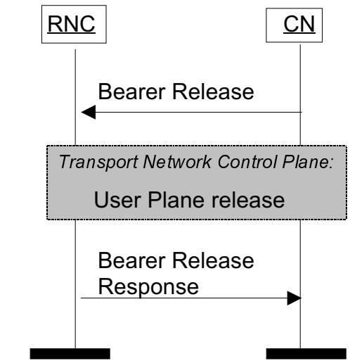
Figure 5. Bearer Release procedure
