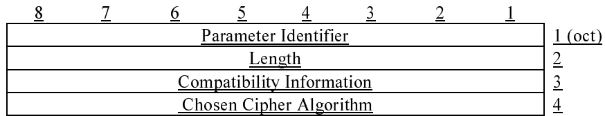
Figure 9.2.4.2-22 format of Chosen Cipher Algorithm
