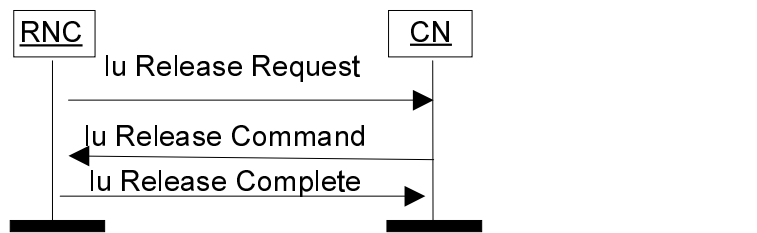
Figure 6. Iu Release: UTRAN generated reasons.
