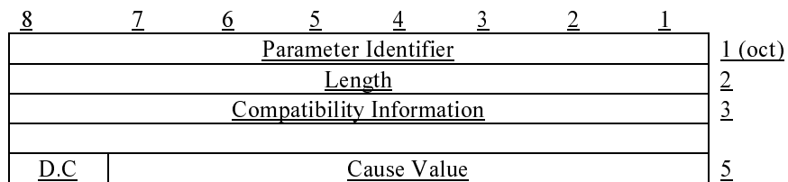
Figure 9.2.4.2-10 format of Cause
