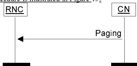
Figure 13. Paging procedure.
