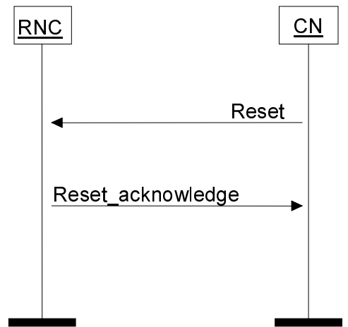
Figure 11. Reset at the CN.
