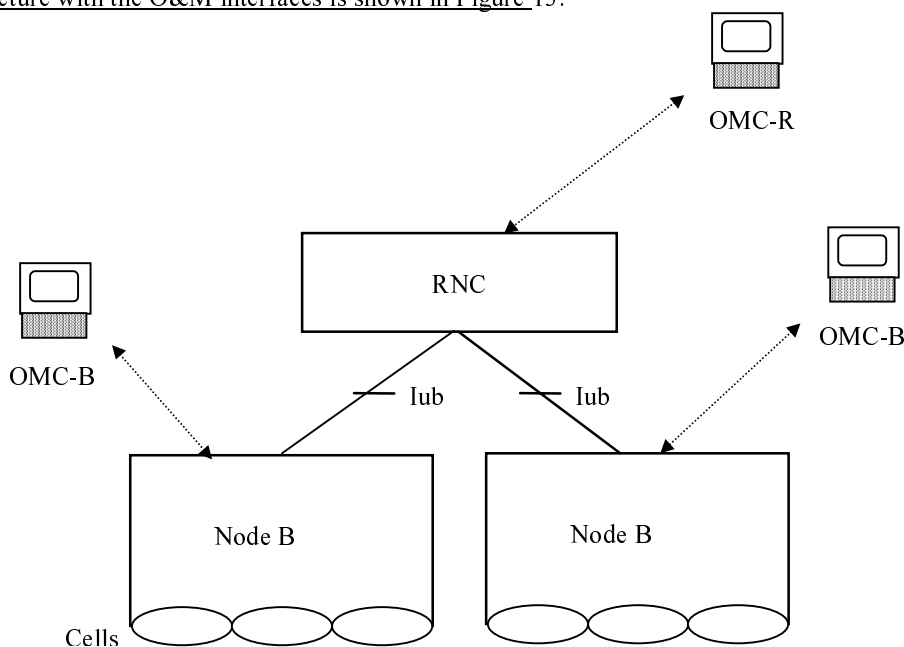
Figure 13. RNS architecture with O&M interfaces
