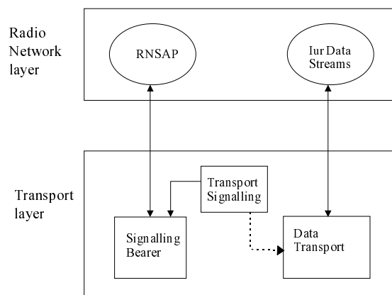
Figure 17. Separation of RNSAP and transport over Iur
