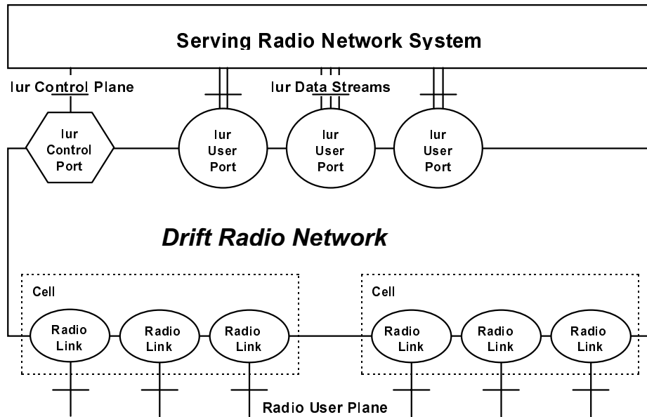
Figure 16. Drift RNS Logical Model
