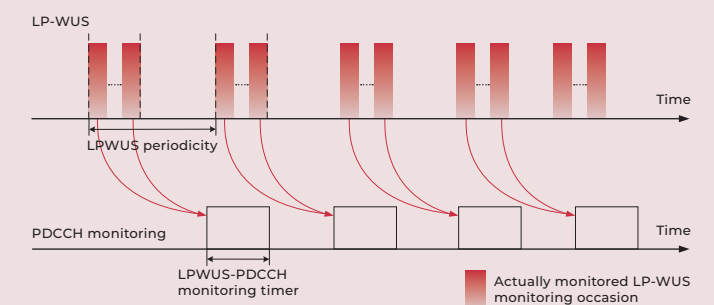
Figure 3 Option 2: LP-WUS operation in RRC connected modeoption 2
