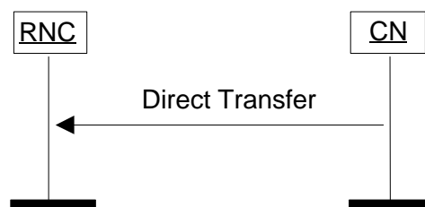
Figure 17. Direct Transfer, CN originated.
