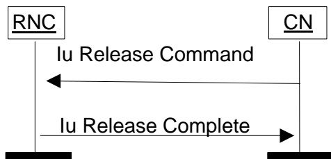
Figure 7. Iu Release: successful handover or SRNS relocation.
