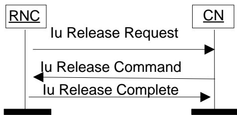
Figure 6. Iu Release: UTRAN generated reasons.
