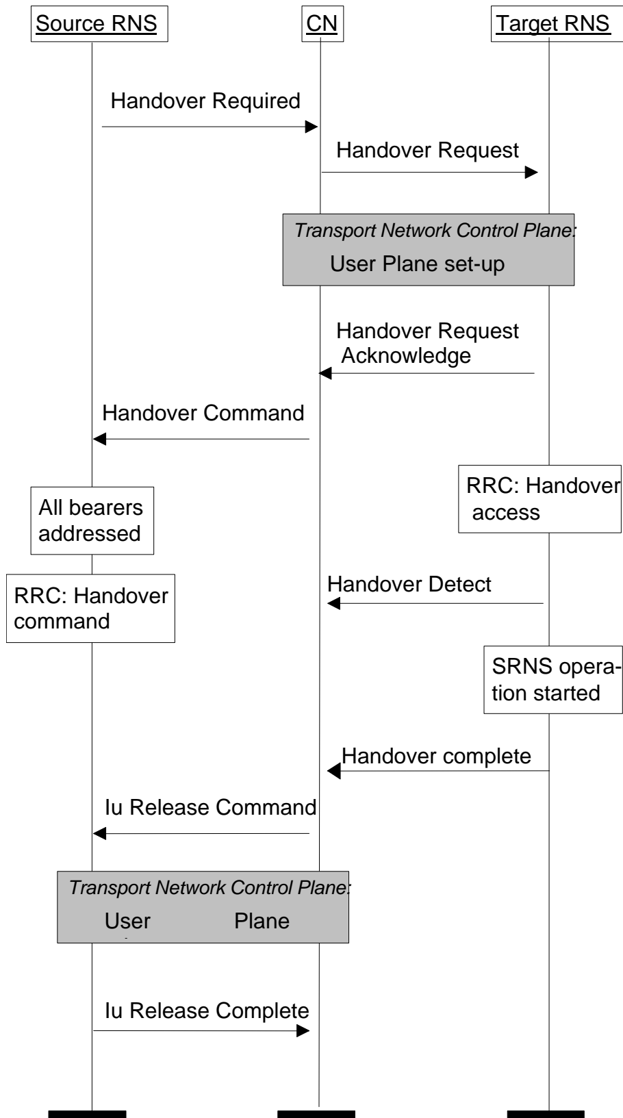
Figure 2. An example RANAP protocol message flow at Iu interface related to Inter RNS Hard Handover. A successful case.
