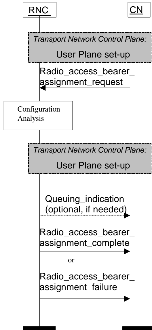
Figure 4. Radio Access Bearer Assignment procedure.
