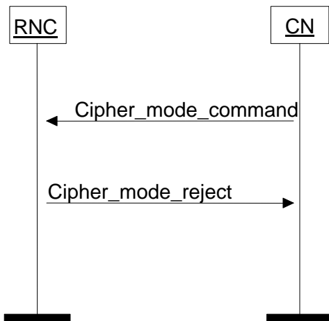
Figure 16. Cipher Mode Control procedure, unsuccessful case.
