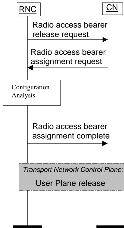
Figure 3. Radio Access Bearer Assignment procedure, UTRAN generated release.
