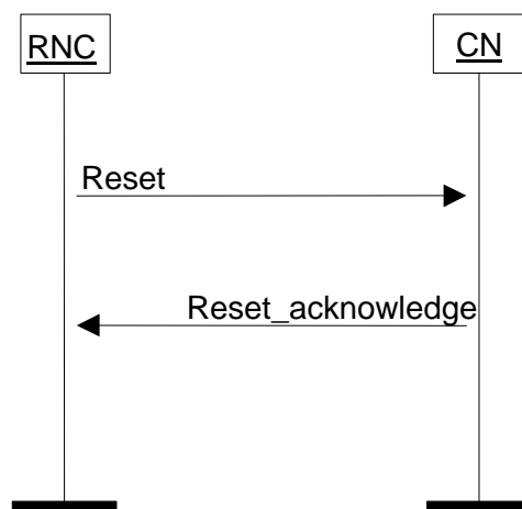
Figure 10. Reset at the UTRAN.
